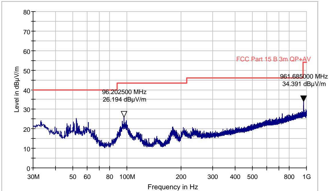
Spurious Emissions 30 – 1000 MHz, Off-Hook, Adaptor PNLV226(FW)
