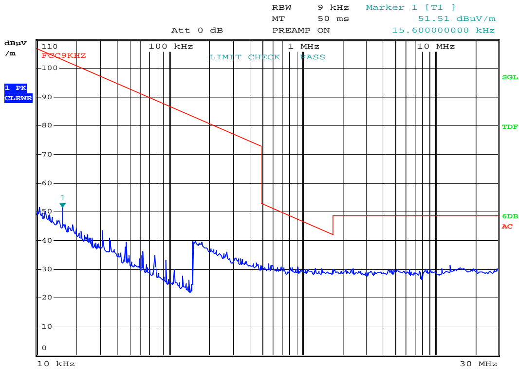
Spurious Emissions 10 kHz – 30 MHz, Adaptor PNLV226(FW)
