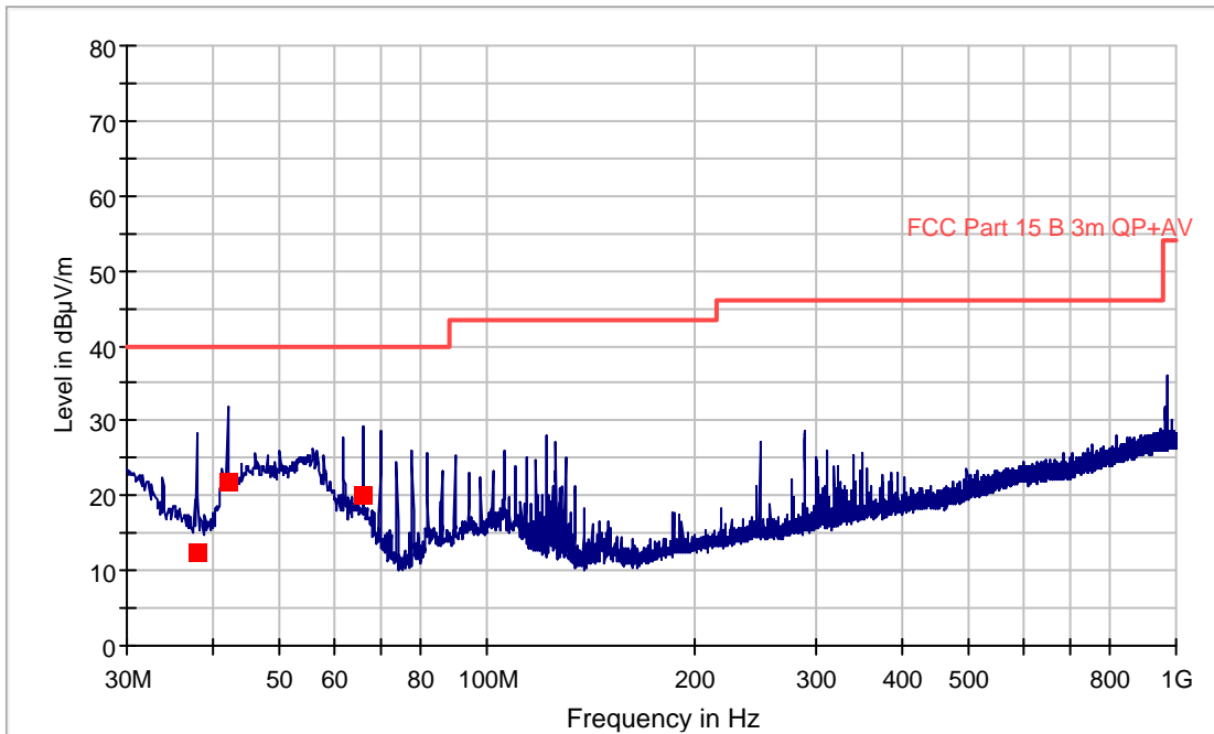
Spurious Emissions 30 - 1000 MHz, Off-Hook, Adaptor PNLV226(UC)
