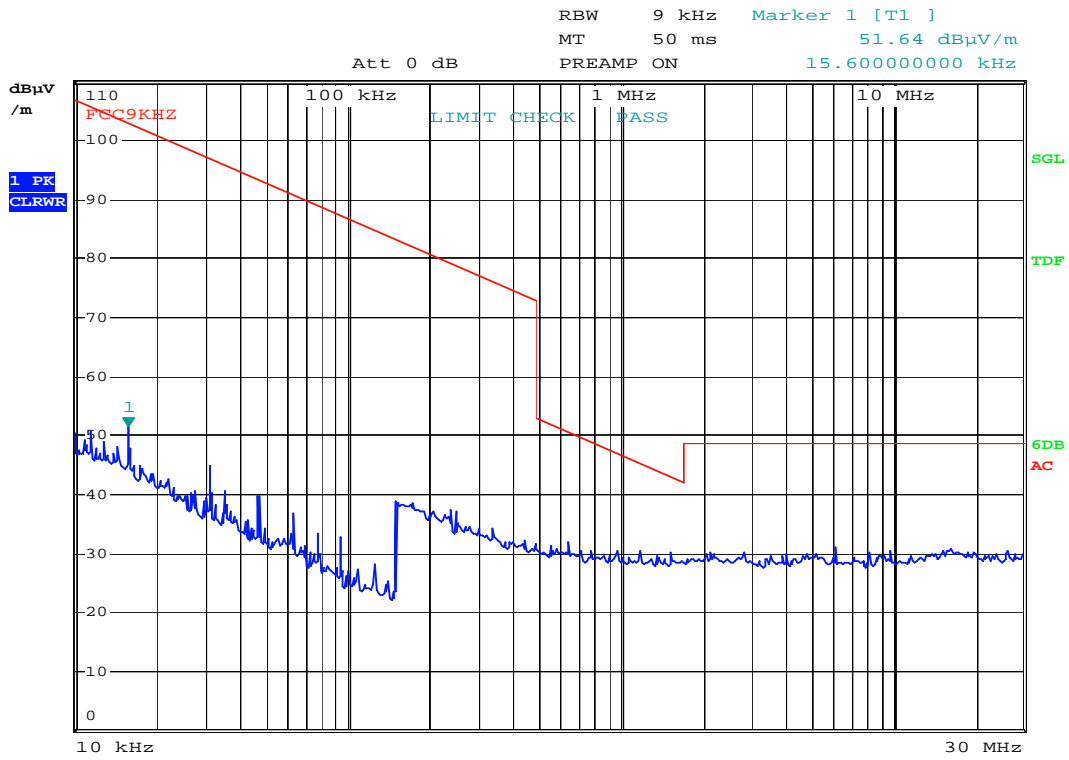
Spurious Emissions 10 kHz – 30 MHz, Adaptor PNLV226(UC)
