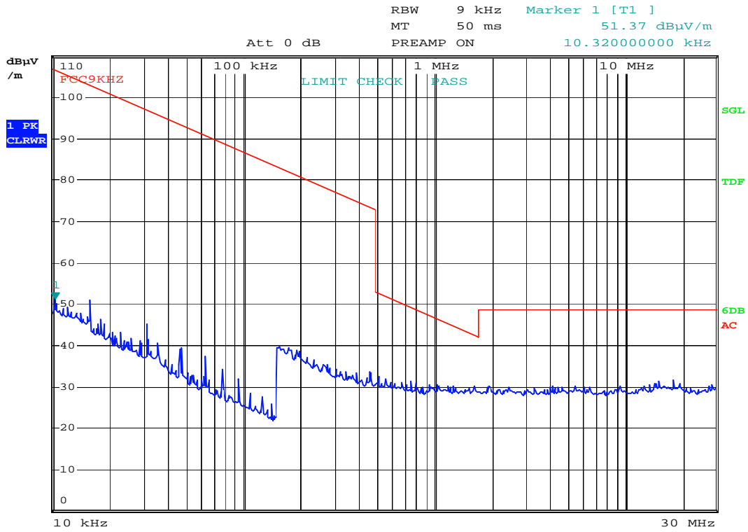
Spurious Emissions 10 kHz – 30 MHz, Adaptor PNLV226(FW)
