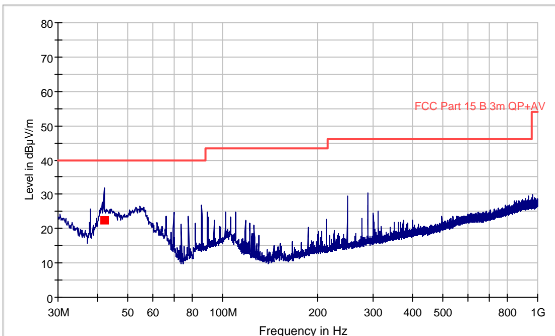
Spurious Emissions 30 - 1000 MHz, On-Hook, Charging, Adaptor PNLV226(UC)
