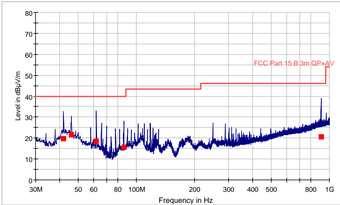
Spurious Emissions 30 – 1000 MHz, Off-Hook, Adaptor PNLV226(FW)
