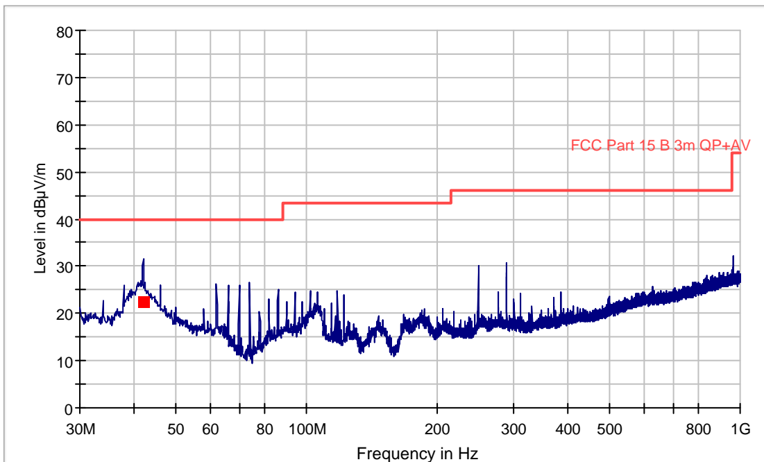
Spurious Emissions 30 – 1000 MHz, On-Hook, Charging, HP Adaptor PNLV226(FW)
