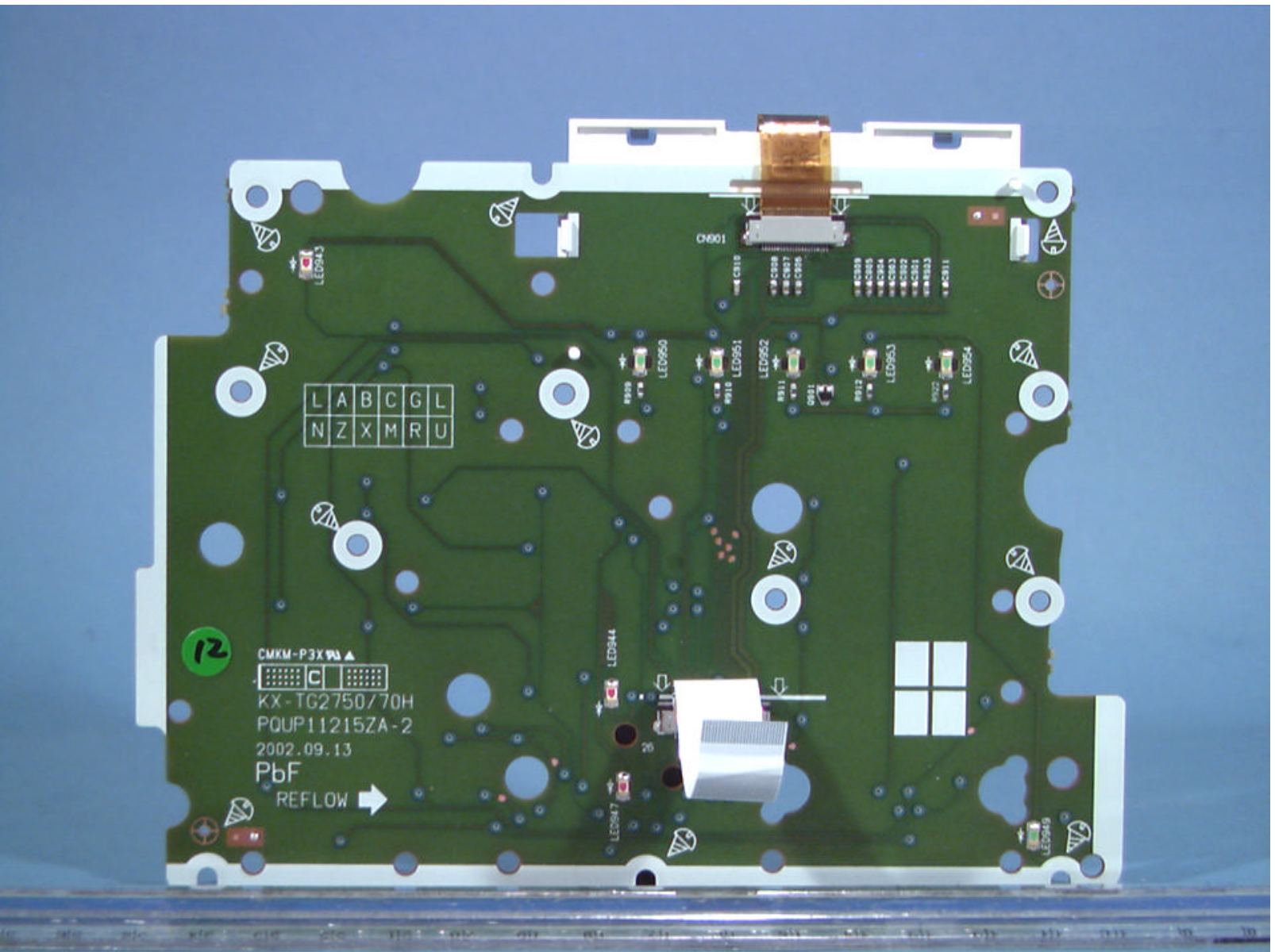
© 2002 PCTEST Lab Panasonic FCC ID: ACJ96NKX-TG2770 2.4 GHz FHSS Cordless Phone (Model: KX-TG2770)
