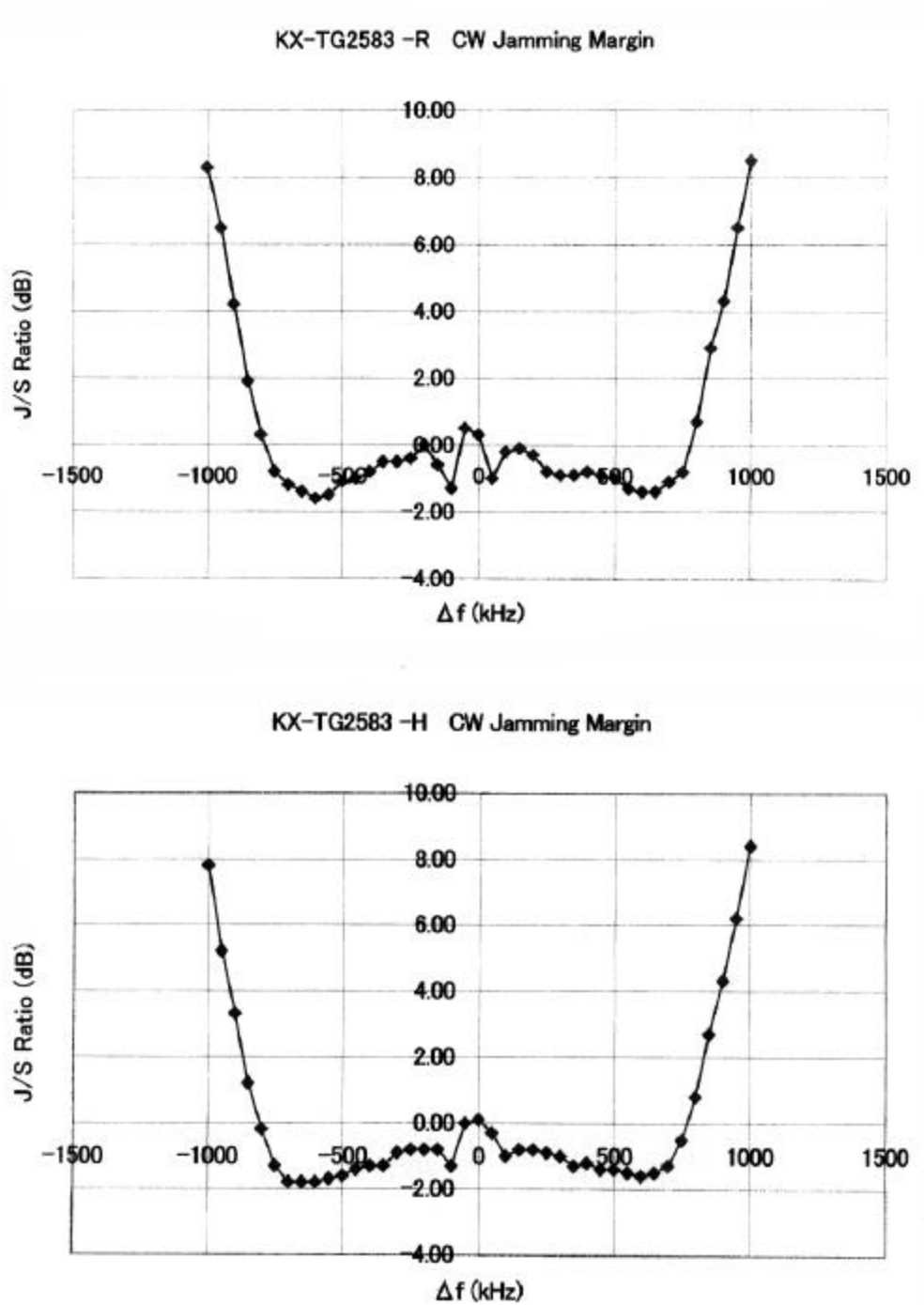
Figure 3: Test Results of Jamming Margin
