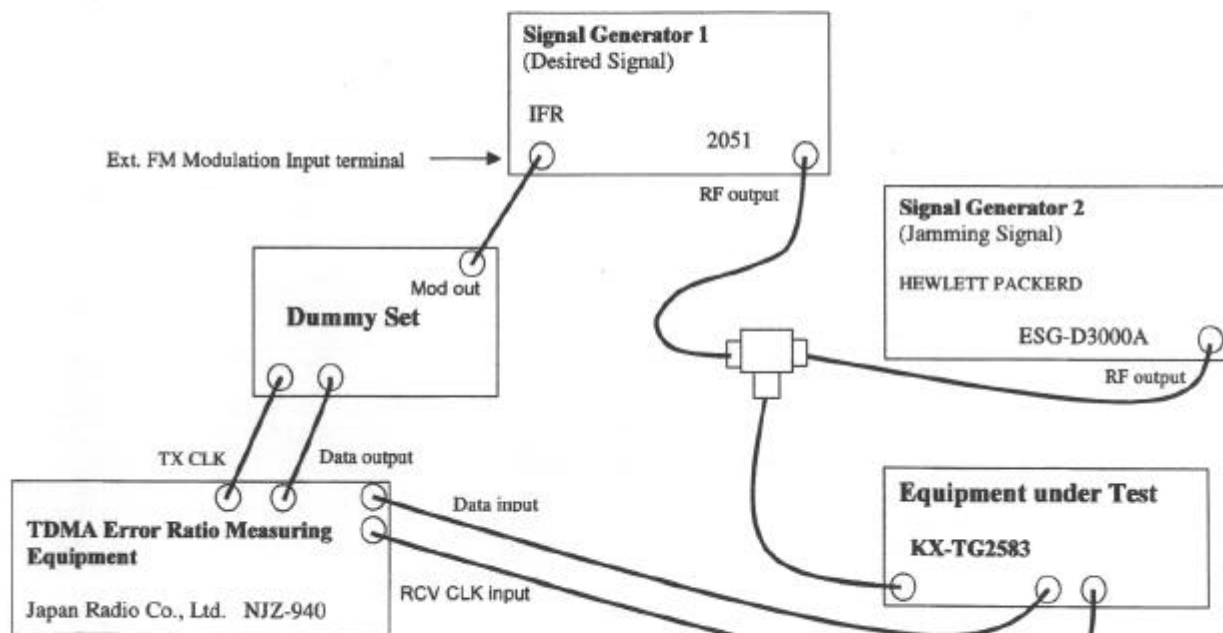
Figure 1: Processing Gain Test Setup
