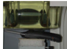
Figure 14.1 Hand Set SAR Test Setup -- 0.5 cm Distance --
