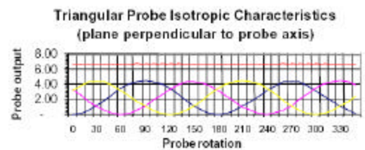
Figure 3.3 Probe Characteristics
