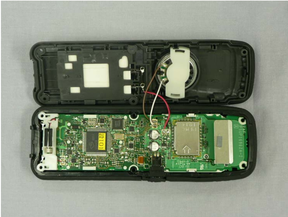
KX-TD7696 Internal view of handset
