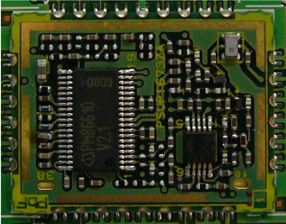
RF module of KX-TD7696, View of under the shield case
