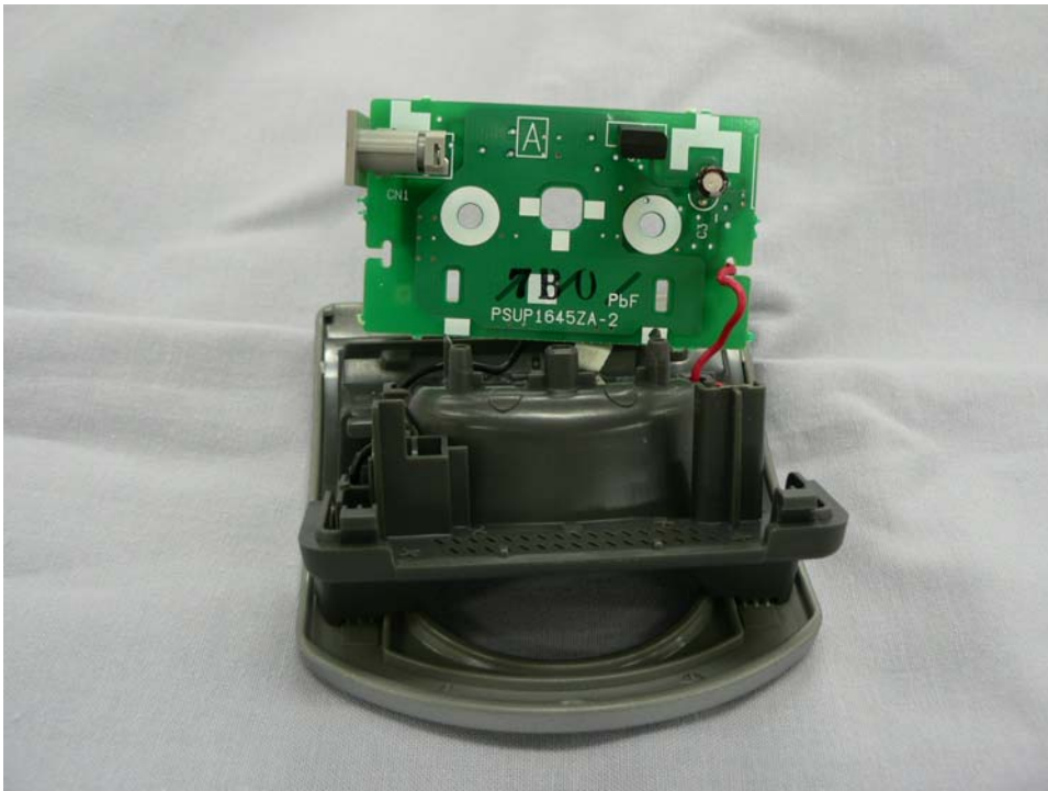
Internal view of battery charger for KX-TD7684
