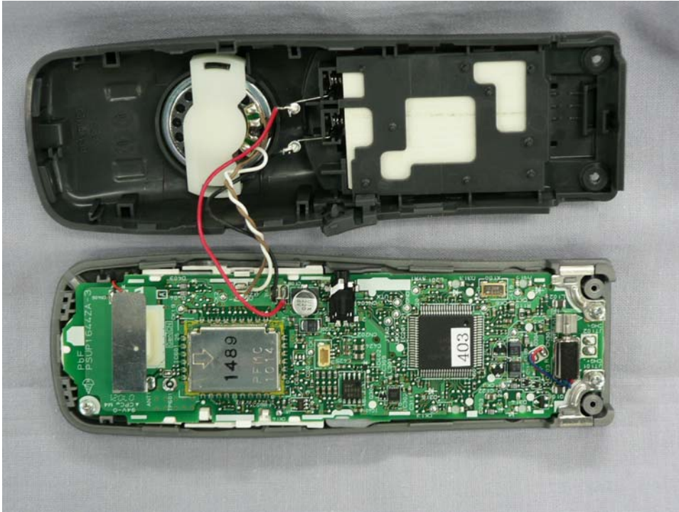
KX-TD7684 Internal view of handset
