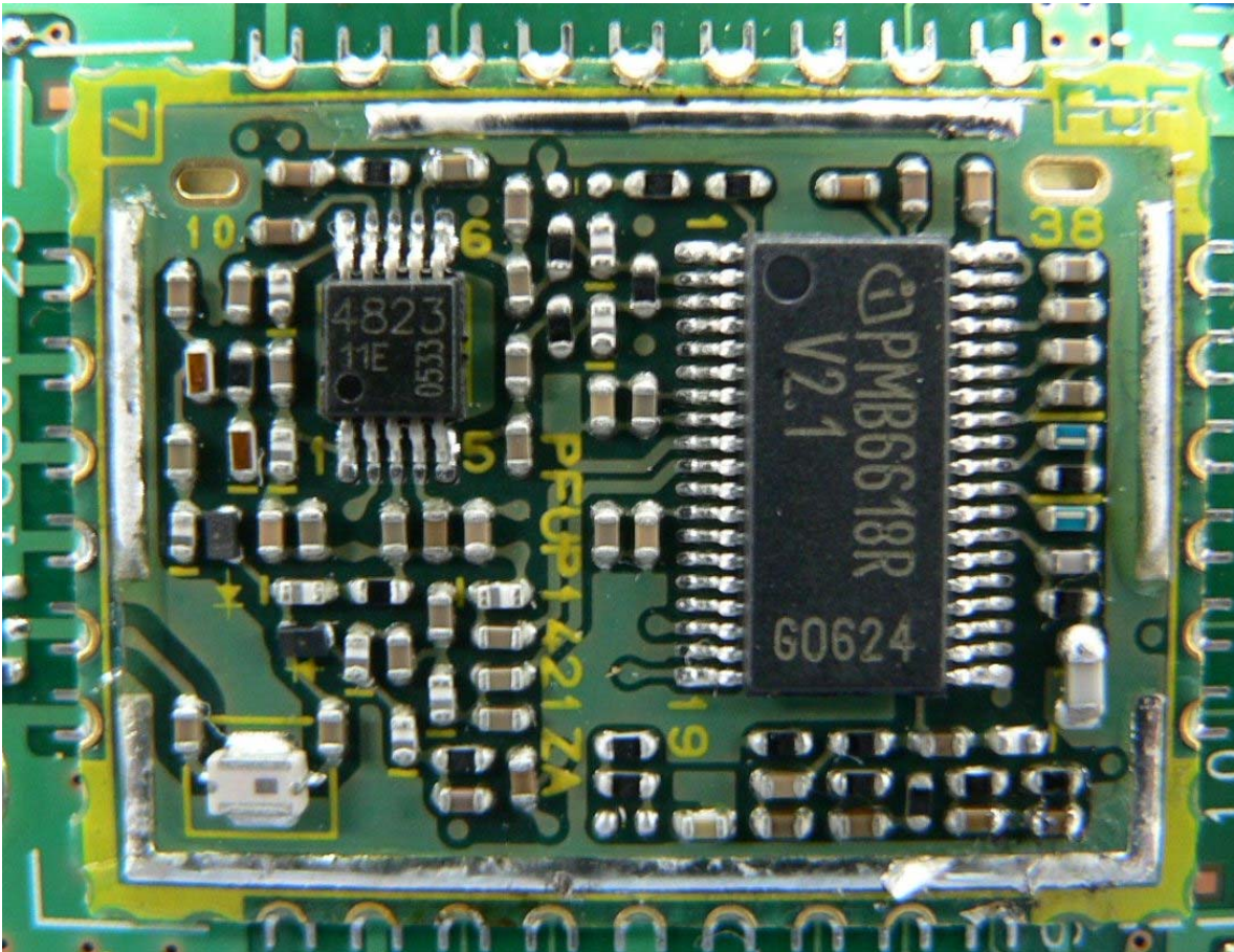
RF module of KX-TD7694 and KX-TD7684, View of under the shield case
