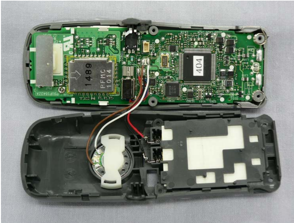
KX-TD7694 Internal view of handset
