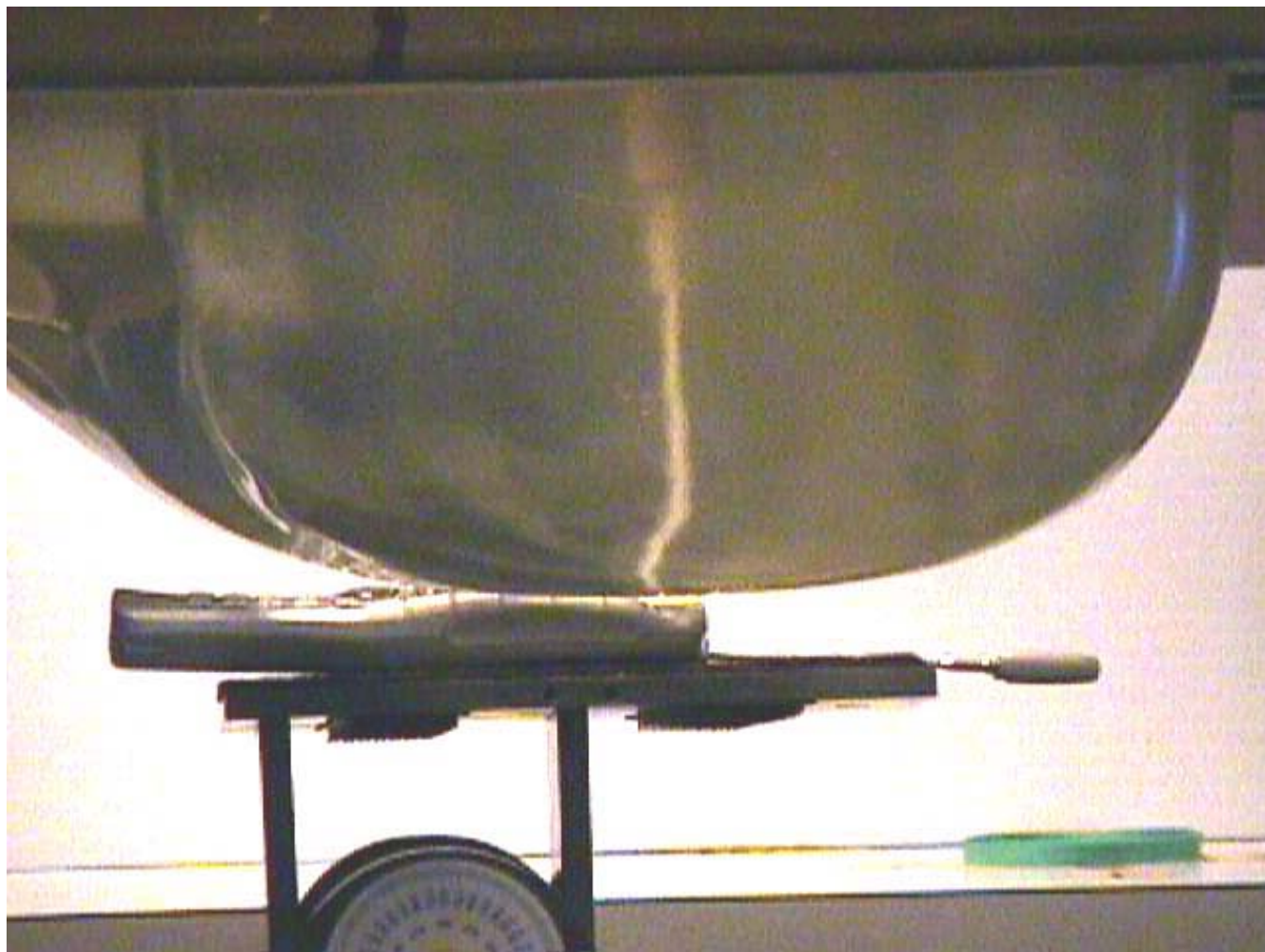
< Left Head, Check Position with the antenna fully extended – Closeup-View >
