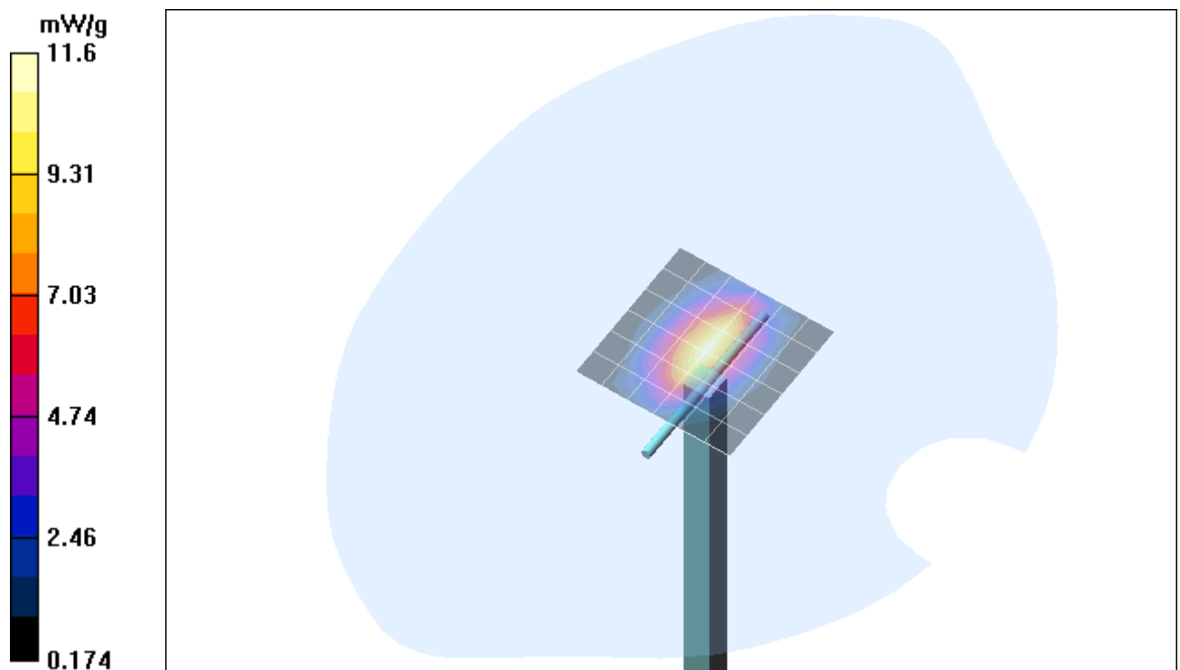
Fig. 9: Validation measurement 1900 MHz body (November 12, 2007), coarse grid. Ambient Temperature: 21.3° C, Liquid Temperature: 20.8° C.
