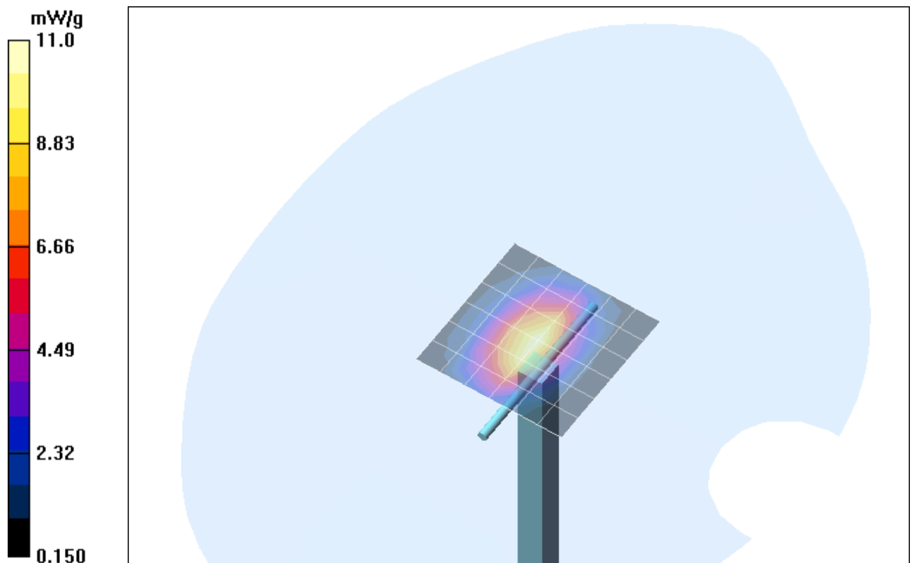
Fig. 8: Validation measurement 1900 MHz Head (November 13, 2007), coarse grid. Ambient Temperature: 21.4° C, Liquid Temperature: 20.7° C.
