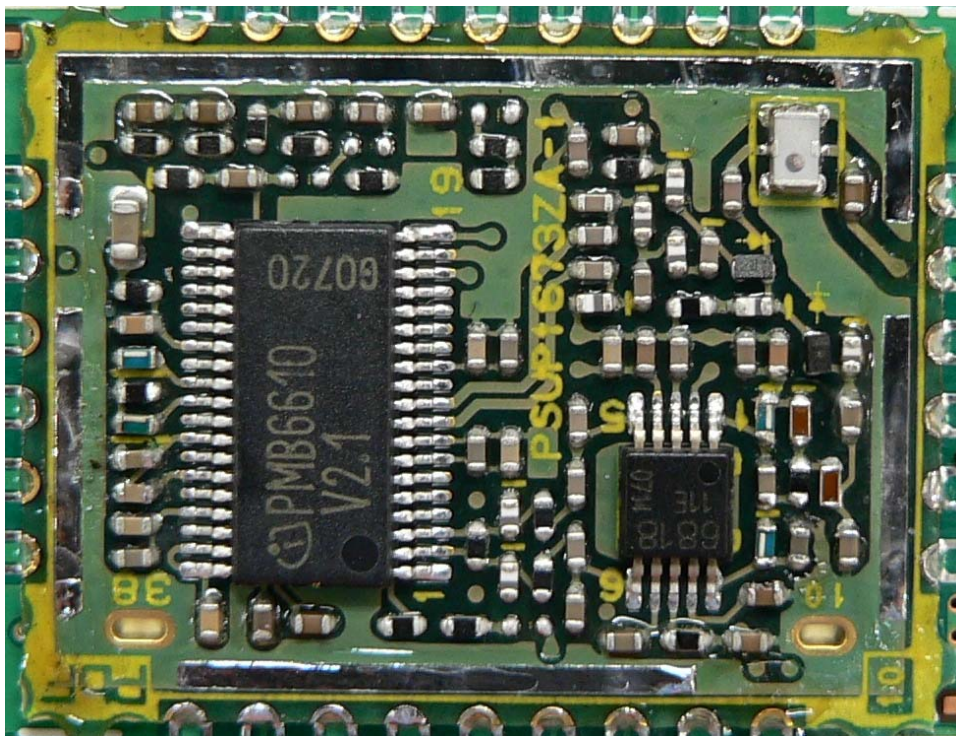
RF module of KX-TD7685 and KX-TD7695, View of under the shield case
