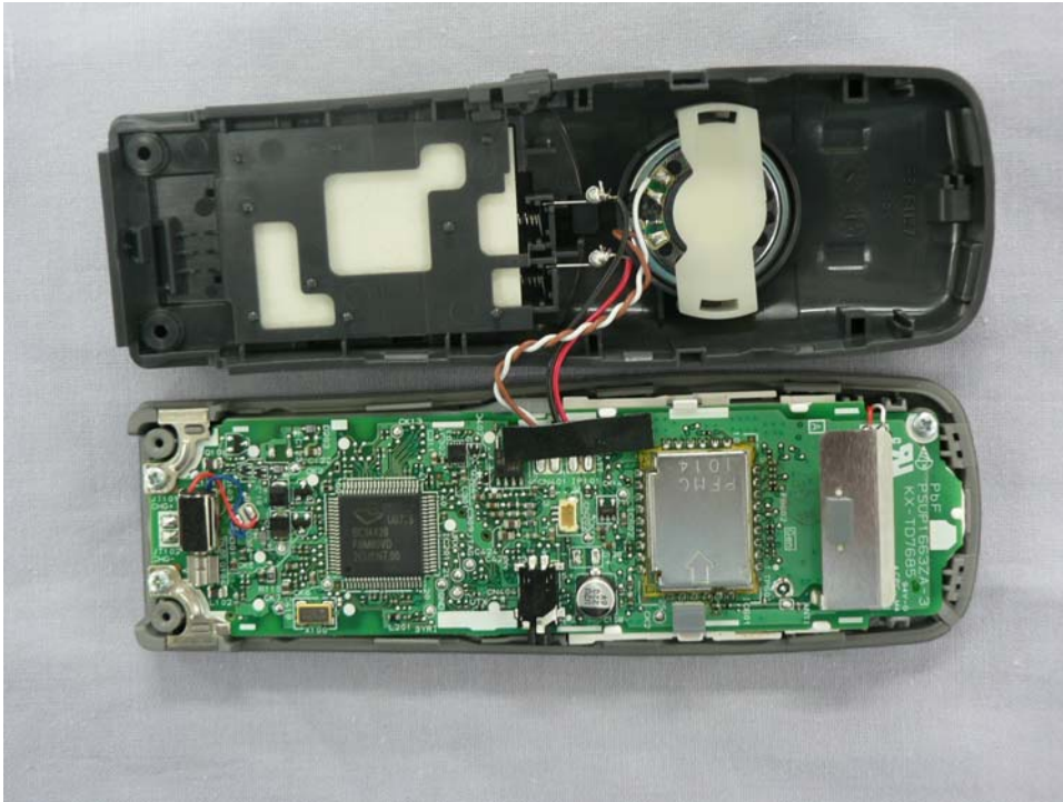
KX-TD7685 Internal view of handset
