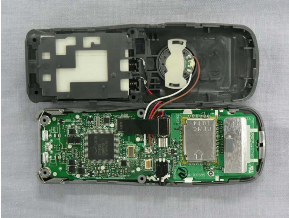
KX-TD7695 Internal view of handset
