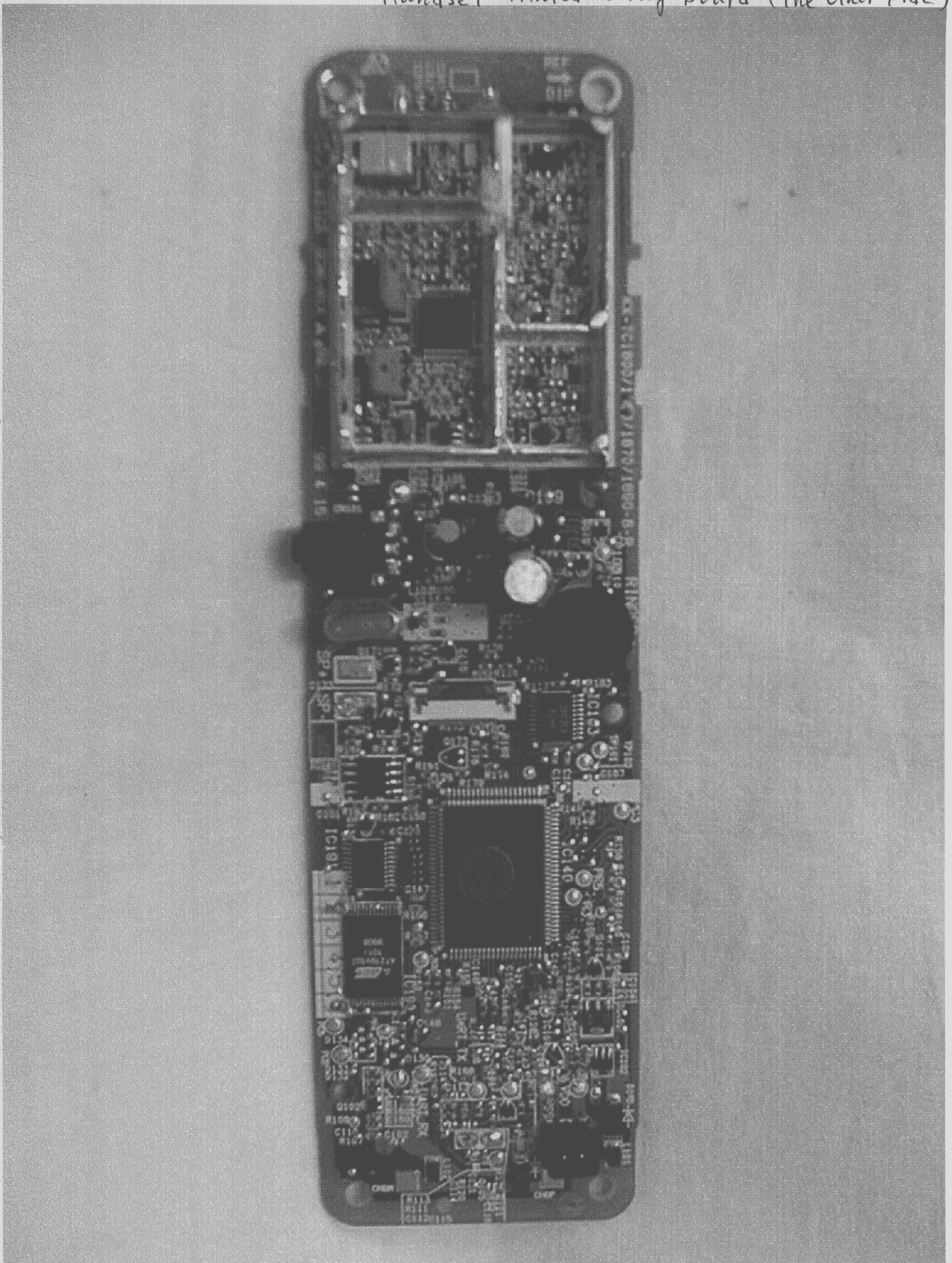
Handset Printed Wiring Board (The Other Side)
