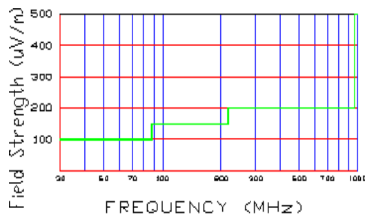
Figure 17. Spurious Radiated Limits at 3 meters
