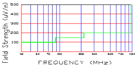
Figure 15. Harmonic Limits at 3 meters
