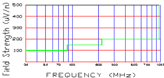
Figure 14. Harmonic Limits at 3 meters
