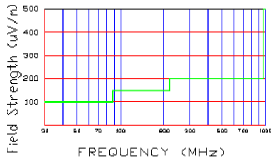
Figure 16. Spurious Radiated Limits at 3 meters
