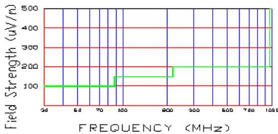
Figure 13. Harmonic Limits at 3 meters
