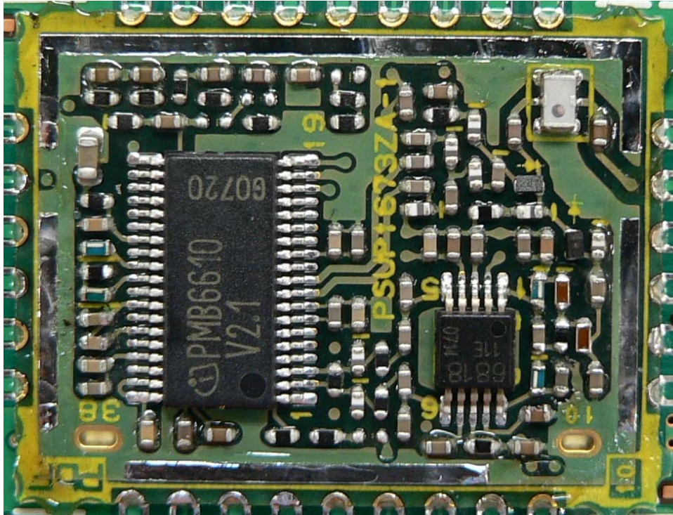
RF module of KX-T0155 and KX-T0158, View of under the shield case
