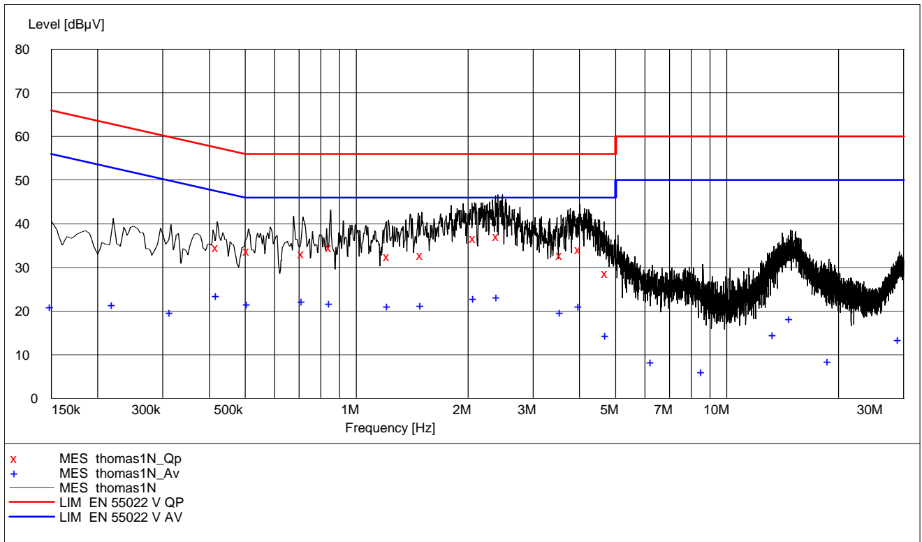
Charging in PNLC1046 Charger with PNLV233 (UC) Adaptor, 120V 60Hz
