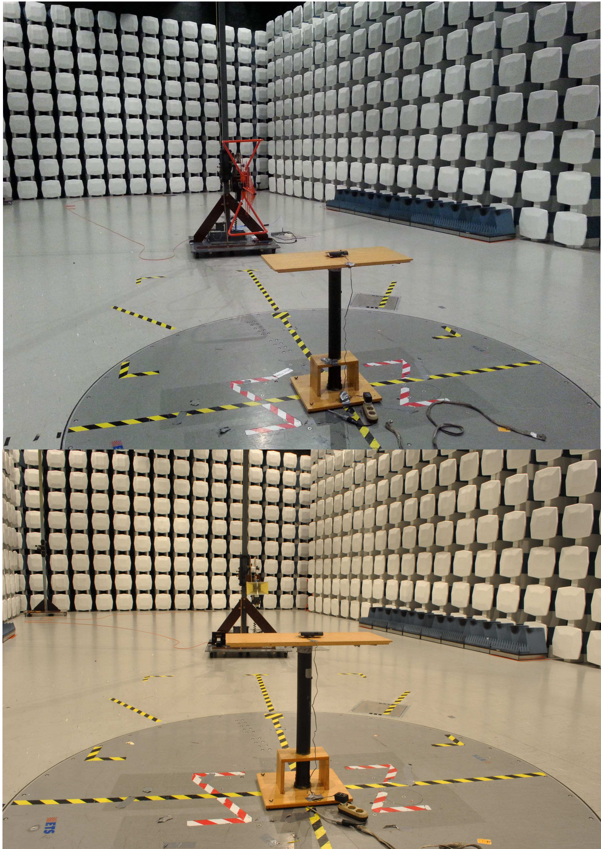
Radiated Emissions Test
