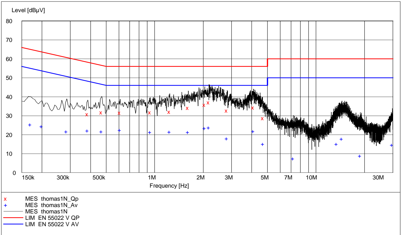
Charging in PNLC1047 Desktop Charger with AC Adaptor PNLV233(UC), 120V 60Hz
