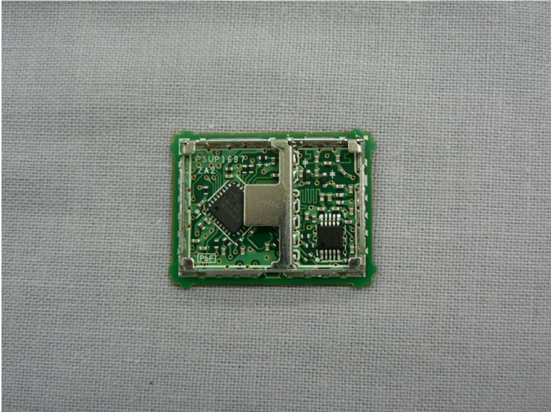
RF module of KX-NCP0158X, View of under the shield case
