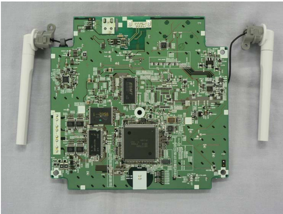
KX-NCP0158X Internal view
