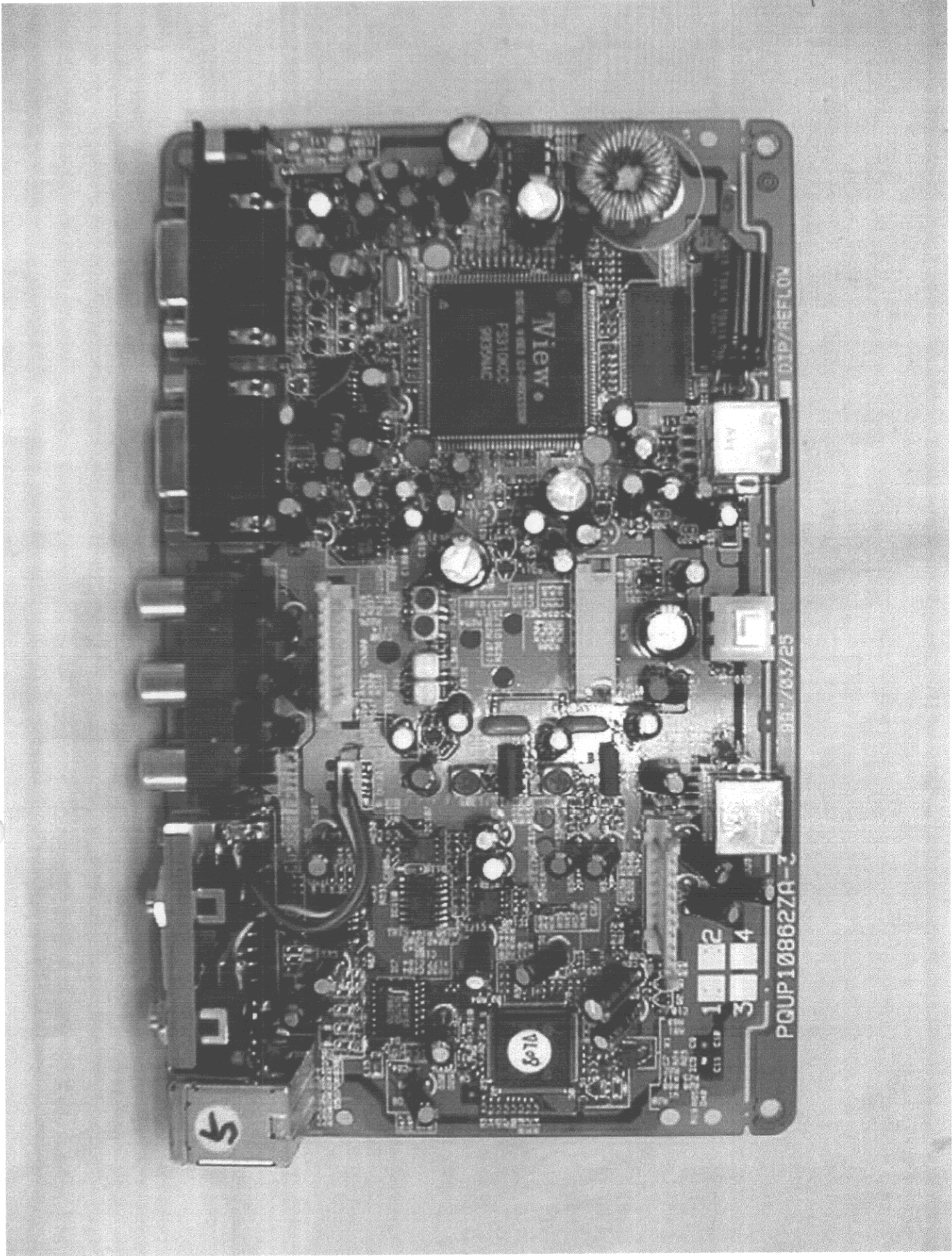
Main Board (Top Side)
