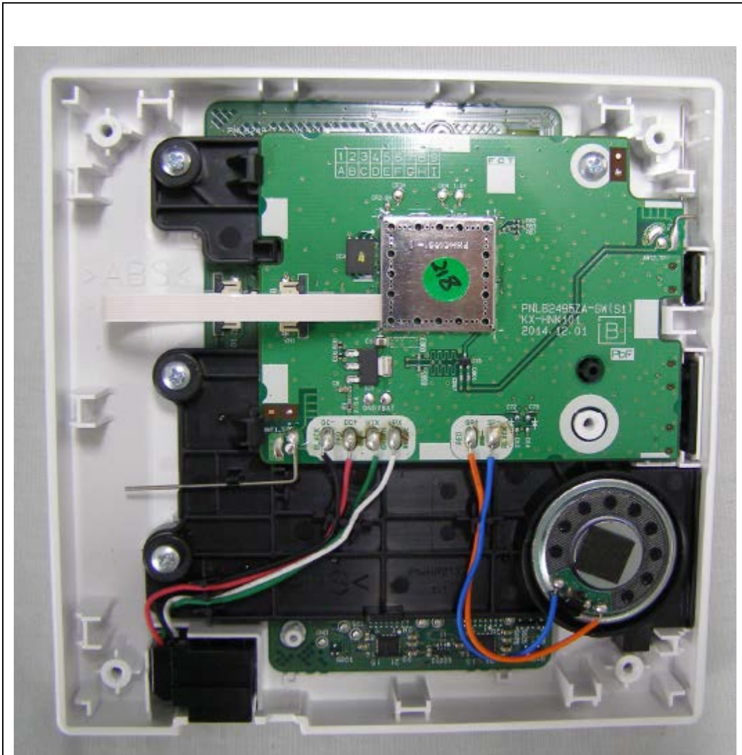
Internal View
