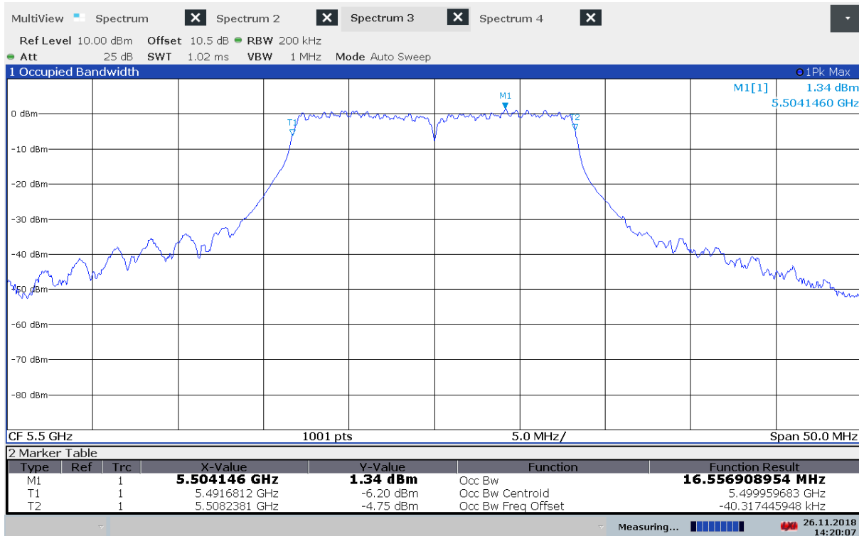
99% Bandwidth, 5500 MHz, 802.11n MCS0
