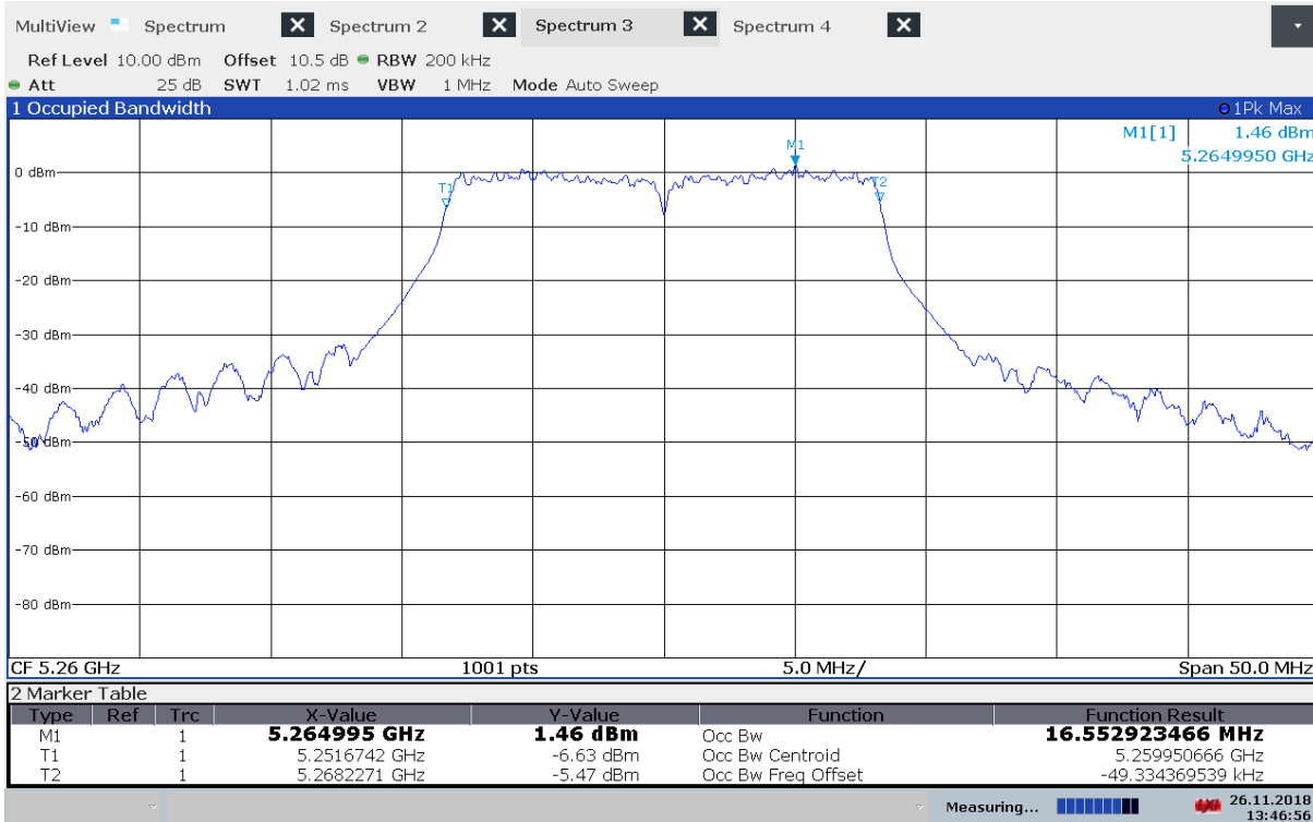
99% Bandwidth, 5260 MHz, 802.11a 6Mbps
