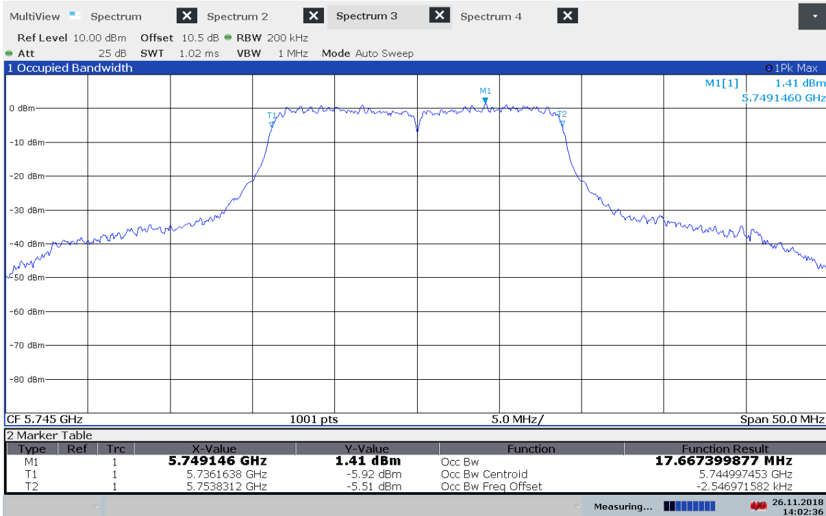
99% Bandwidth, 5745 MHz, 802.11a 6Mbps
