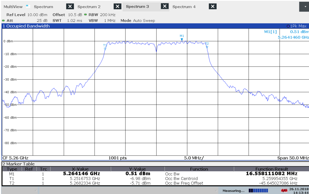
99% Bandwidth, 5260 MHz, 802.11n MCS0
