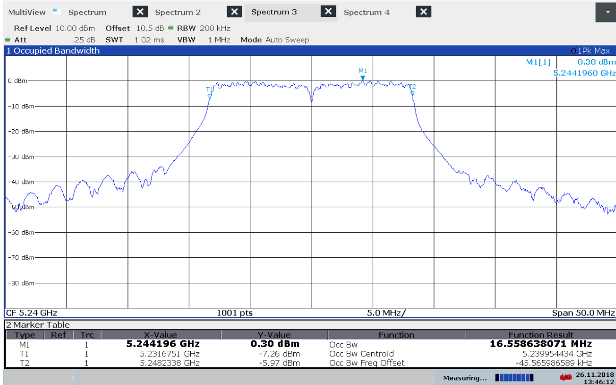
99% Bandwidth, 5240 MHz, 802.11a 6Mbps
