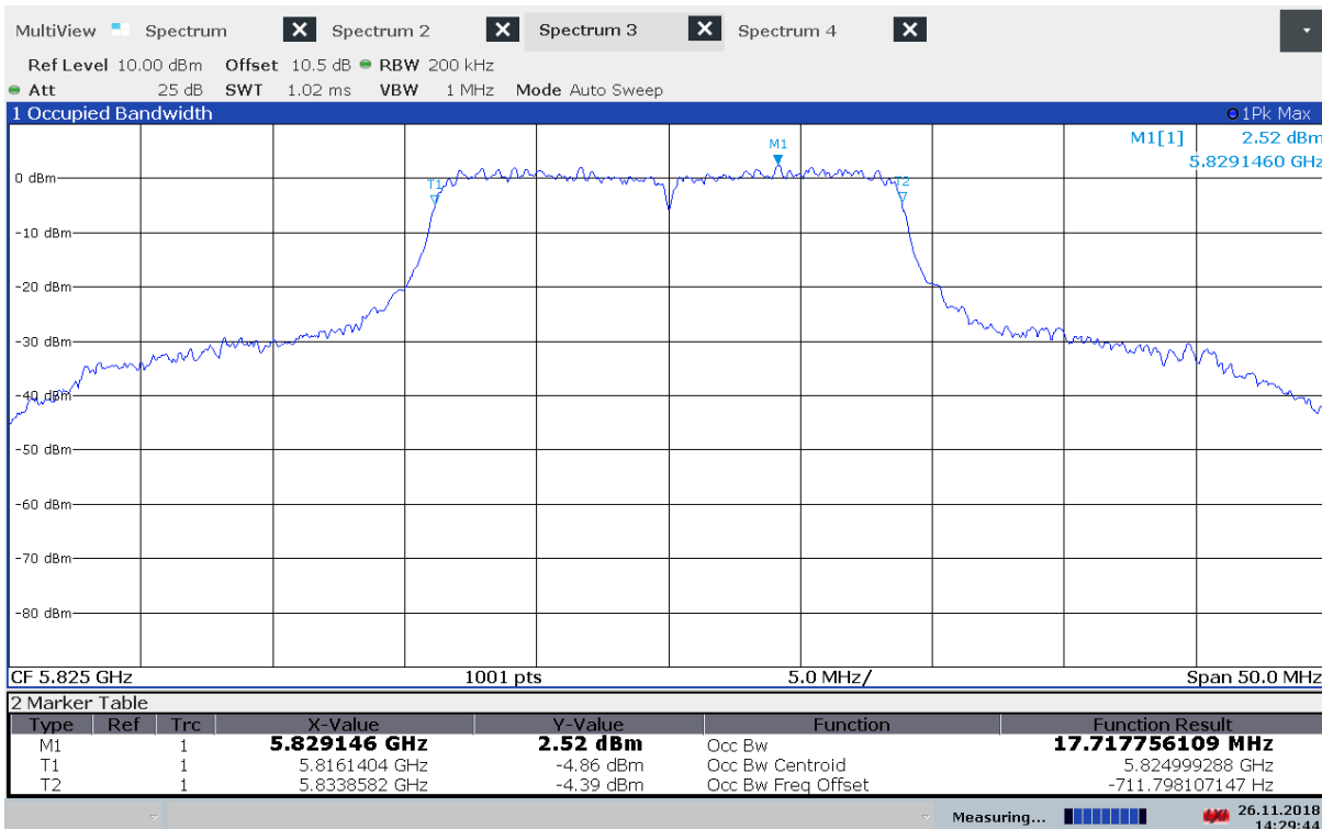
99% Bandwidth, 5825 MHz, 802.11n MCS0
