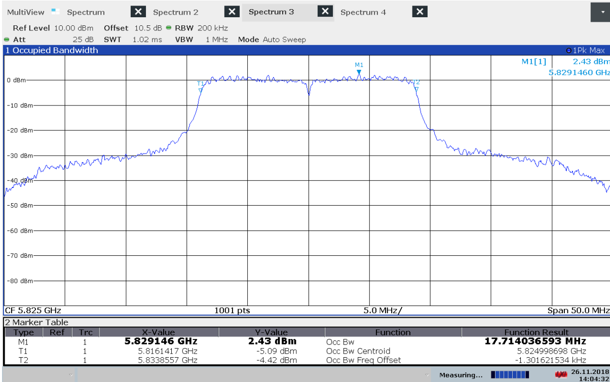
99% Bandwidth, 5825 MHz, 802.11a 6Mbps
