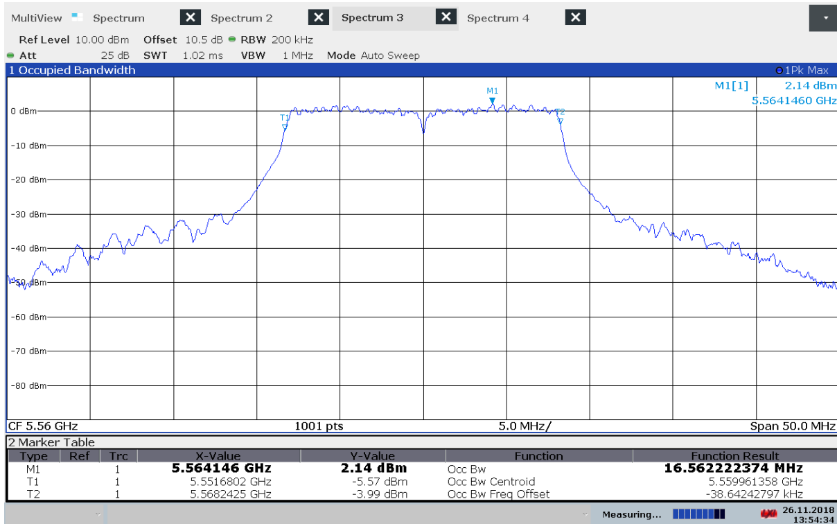
99% Bandwidth, 5560 MHz, 802.11a 6Mbps
