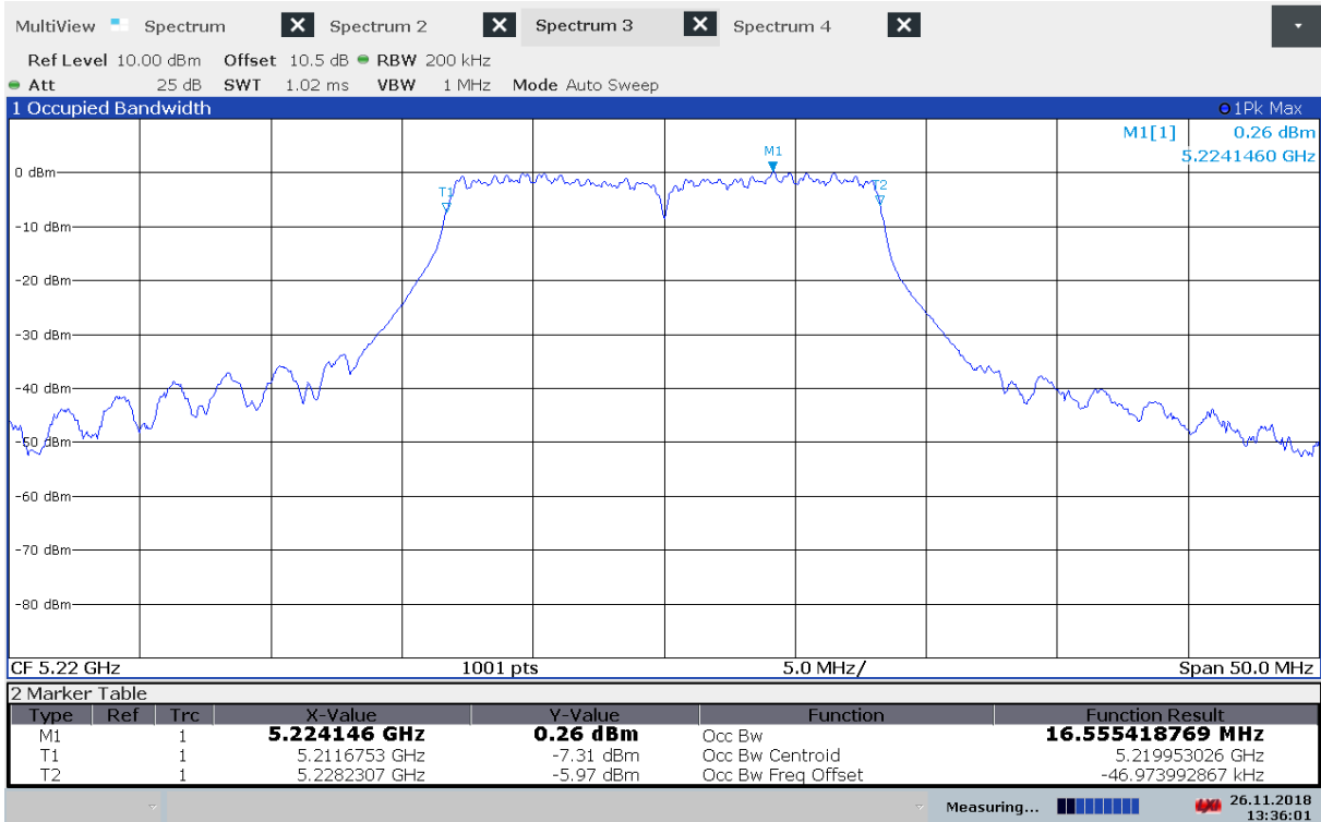
99% Bandwidth, 5220 MHz, 802.11a 6Mbps
