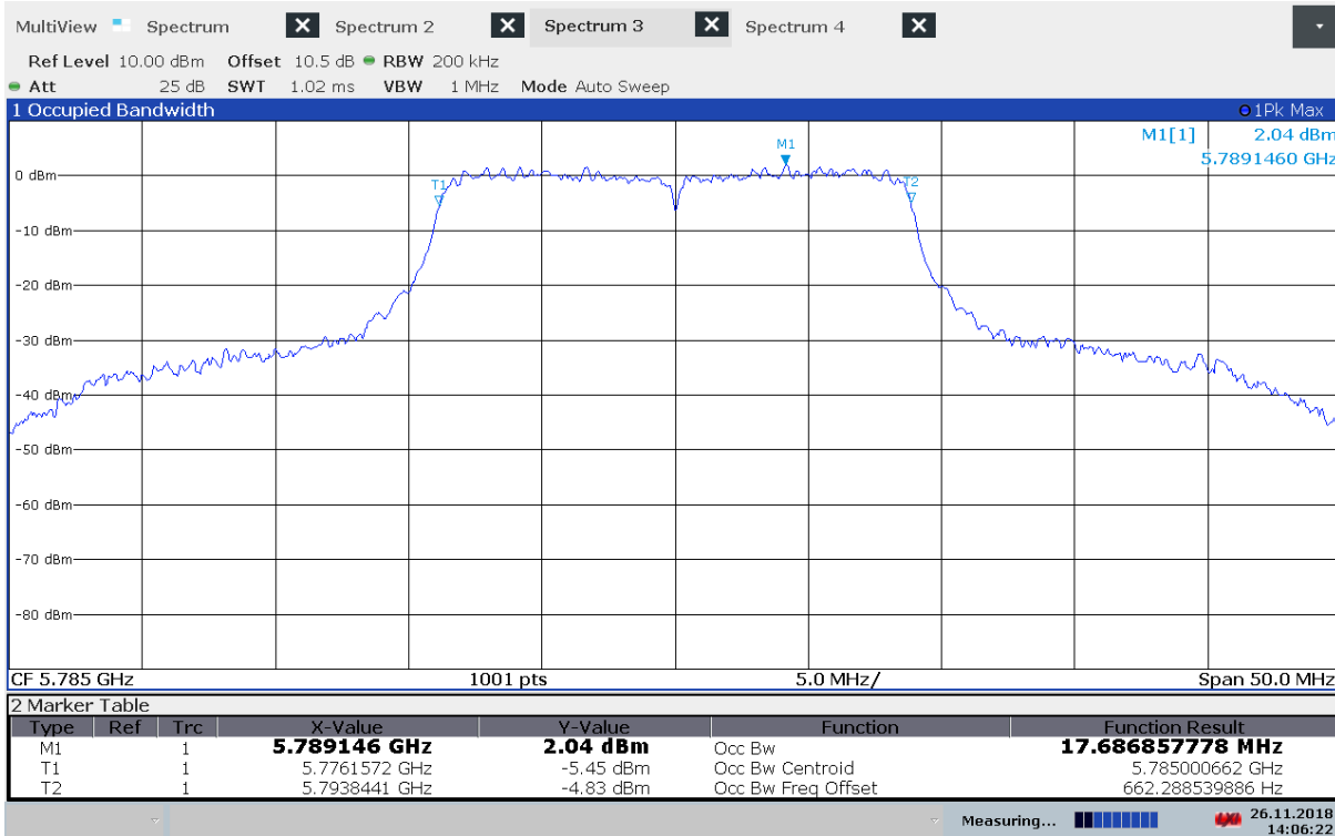
99% Bandwidth, 5785 MHz, 802.11a 6Mbps
