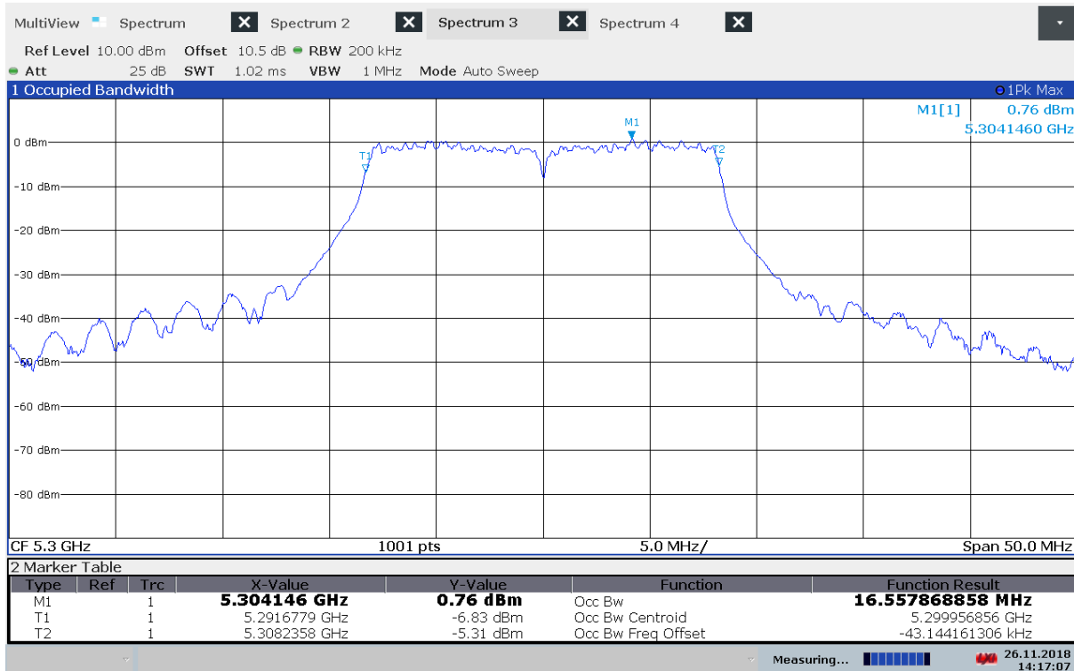
99% Bandwidth, 5300 MHz, 802.11n MCS0
