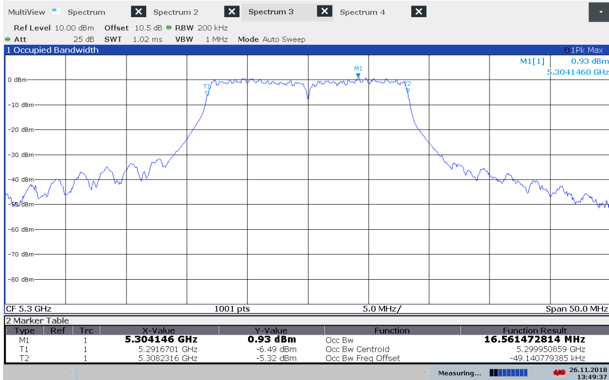
99% Bandwidth, 5300 MHz, 802.11a 6Mbps
