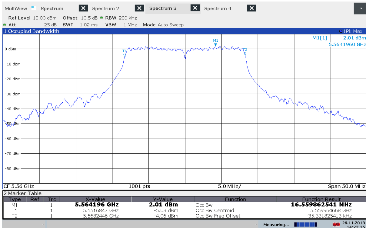
99% Bandwidth, 5560 MHz, 802.11n MCS0
