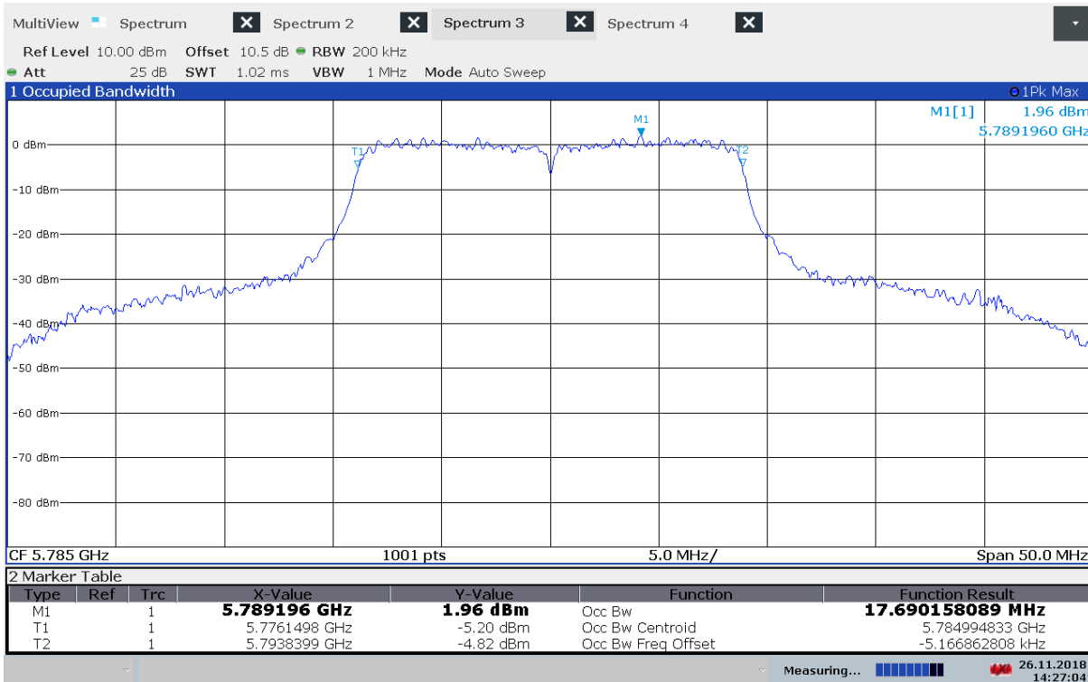
99% Bandwidth, 5785 MHz, 802.11n MCS0
