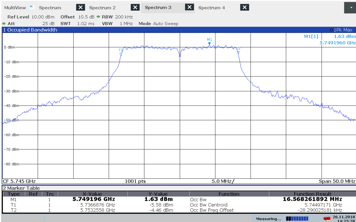
99% Bandwidth, 5745 MHz, 802.11n MCS0
