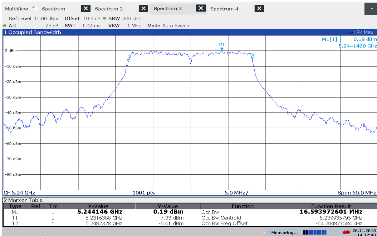
99% Bandwidth, 5240 MHz, 802.11n MCS0
