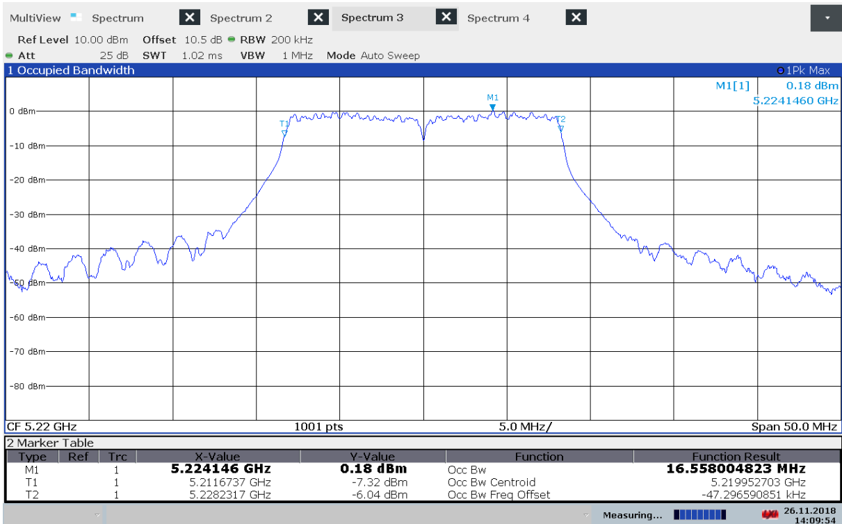
99% Bandwidth, 5220 MHz, 802.11n MCS0
