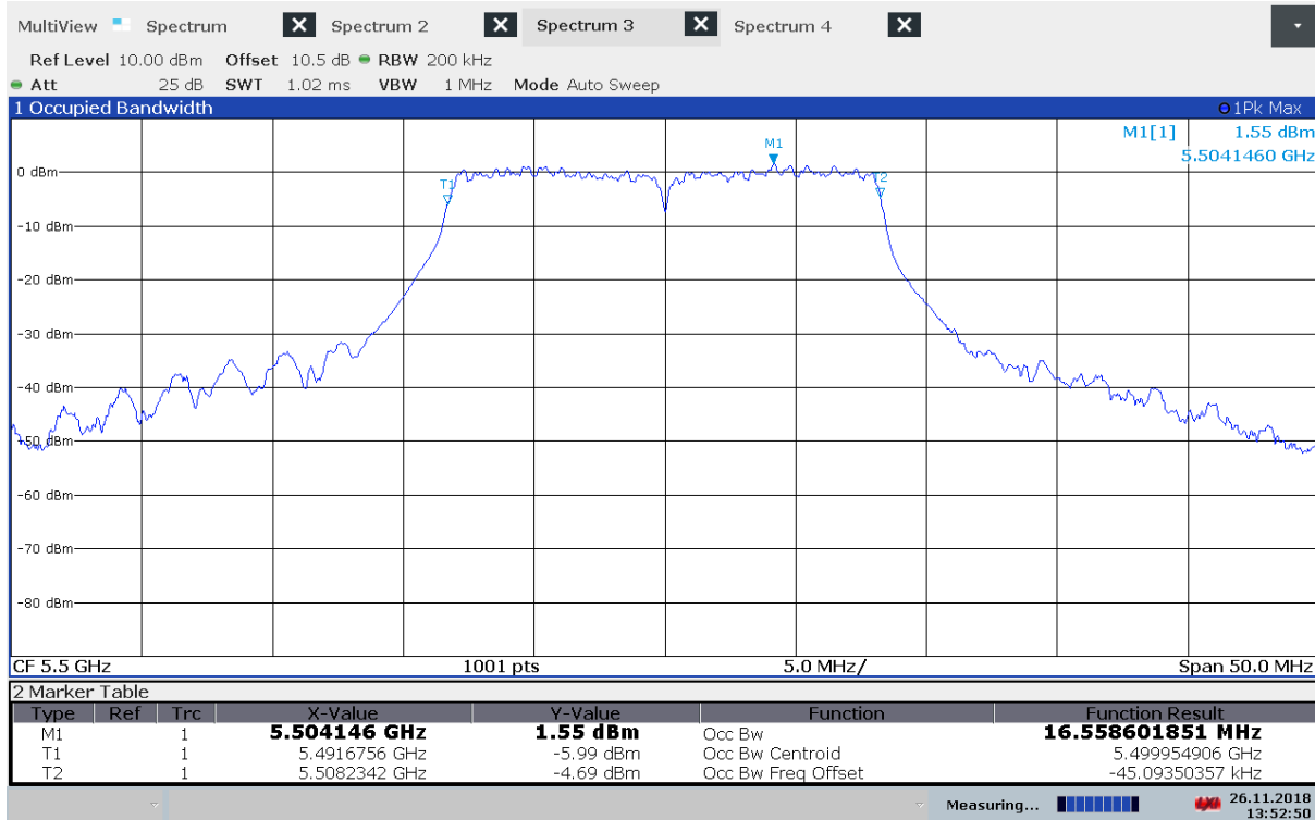
99% Bandwidth, 5500 MHz, 802.11a 6Mbps
