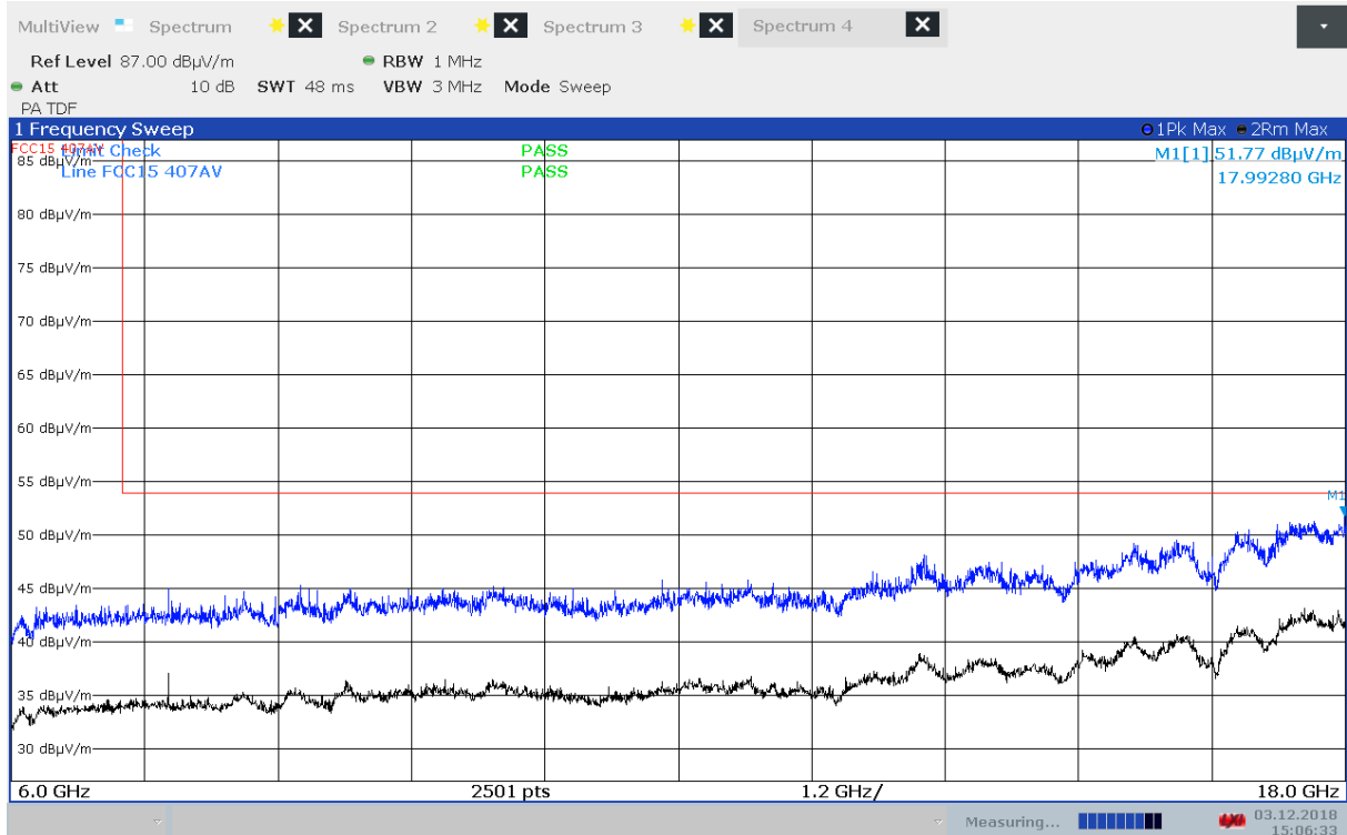
Radiated Emissions, 6000 - 18000 MHz, 5560 MHz, 802.11a 6Mbps, EUT V, VP
