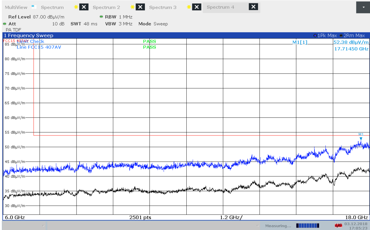
Radiated Emissions, 6000 - 18000 MHz, 5500 MHz, 802.11n MCS0, EUT V, VP
