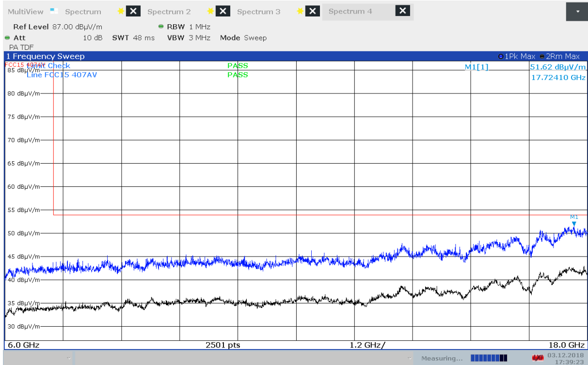
Radiated Emissions, 6000 - 18000 MHz, 5700 MHz, 802.11n MCS0, EUT V, VP
