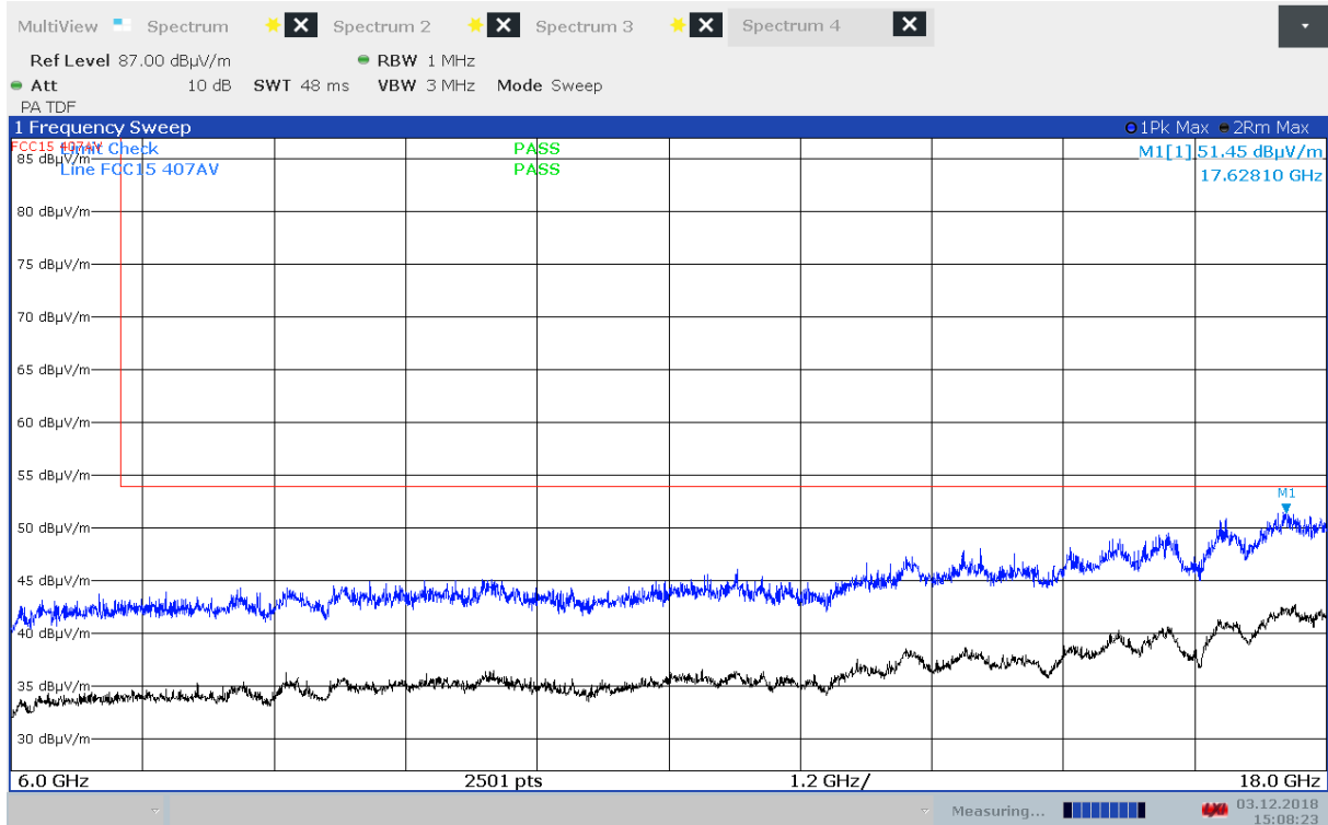
Radiated Emissions, 6000 - 18000 MHz, 5560 MHz, 802.11a 6Mbps, EUT V, HP
