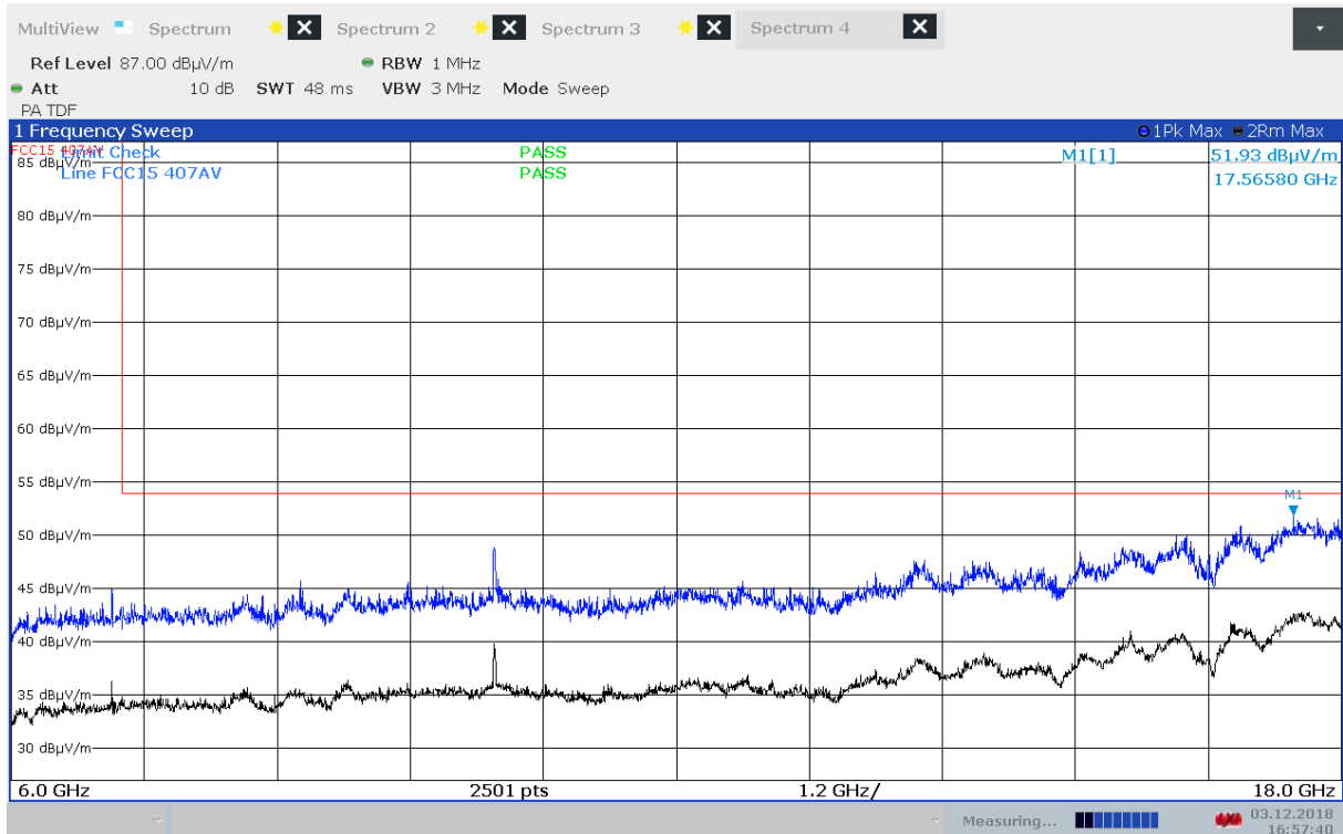
Radiated Emissions, 6000 - 18000 MHz, 5180 MHz, 802.11n MCS0, EUT V, VP
