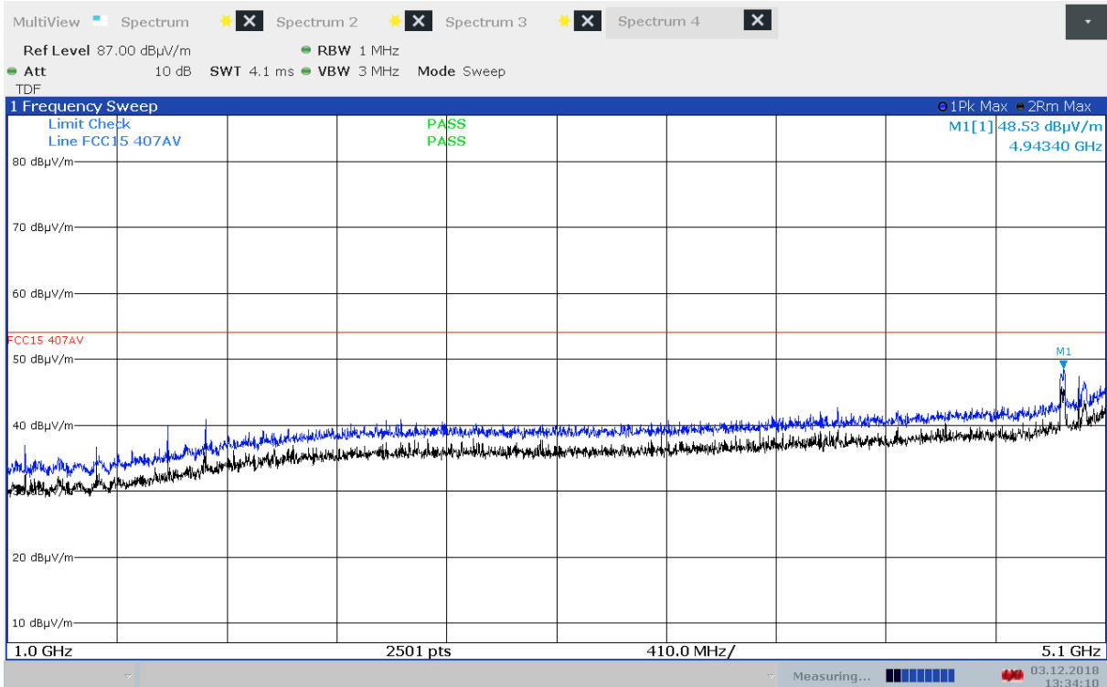
Radiated Emissions, 1000 - 5100 MHz, 5180 MHz, 802.11n MCS0, EUT V, VP
