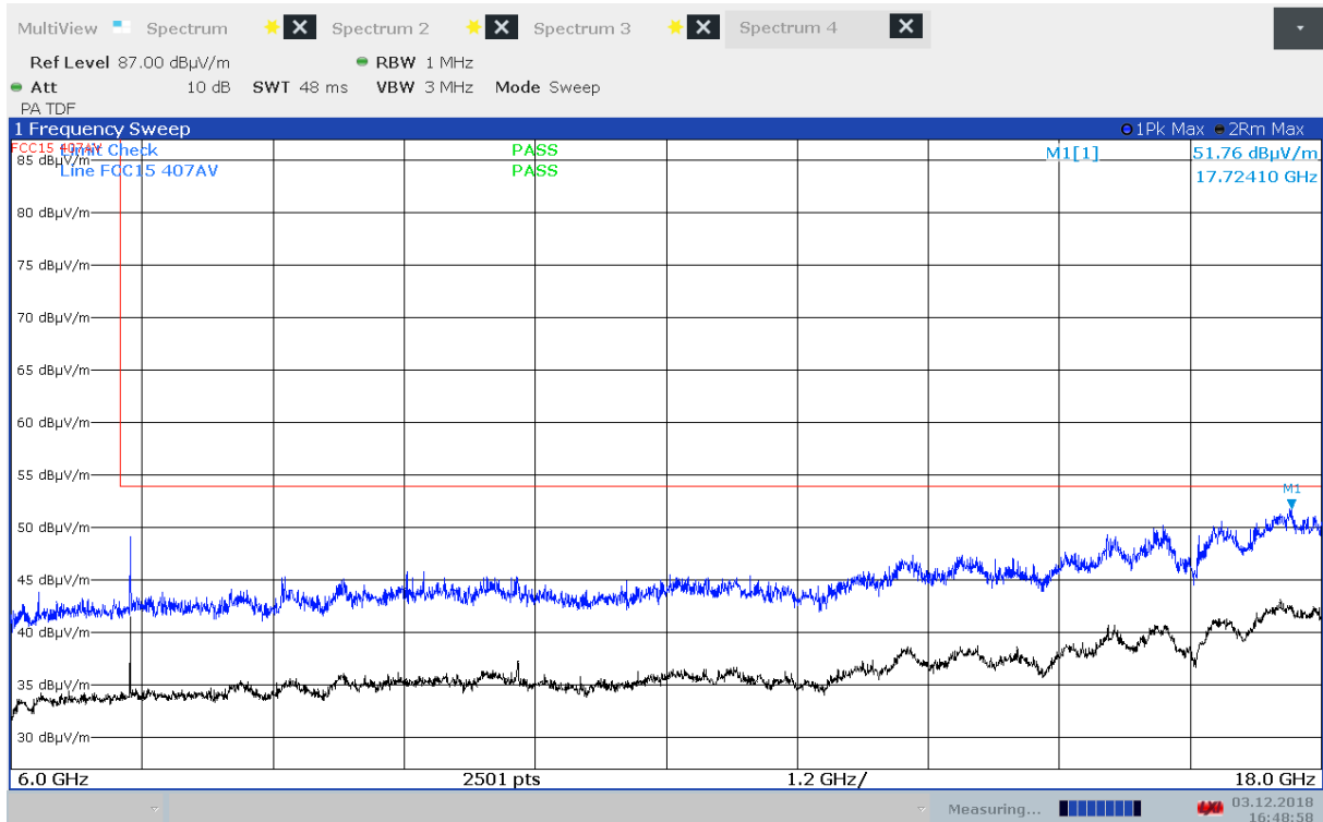
Radiated Emissions, 6000 - 18000 MHz, 5320 MHz, 802.11n MCS0, EUT V, VP
