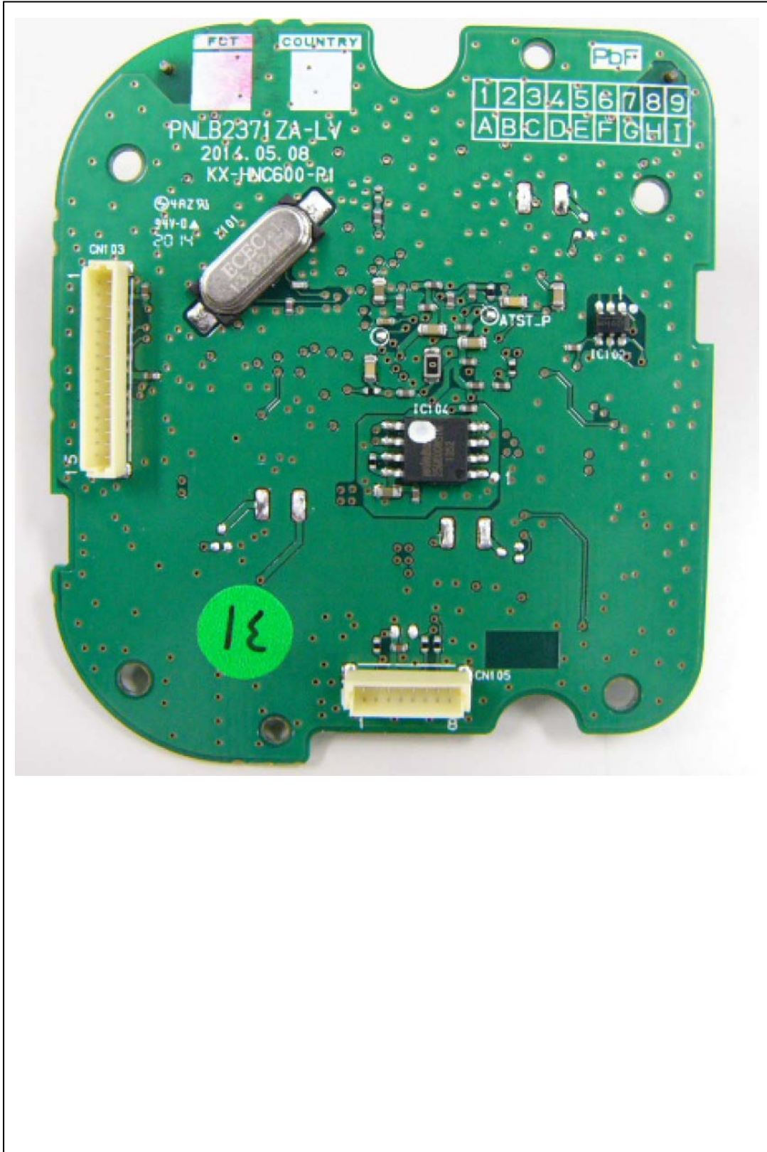
Main Board (Downside)
