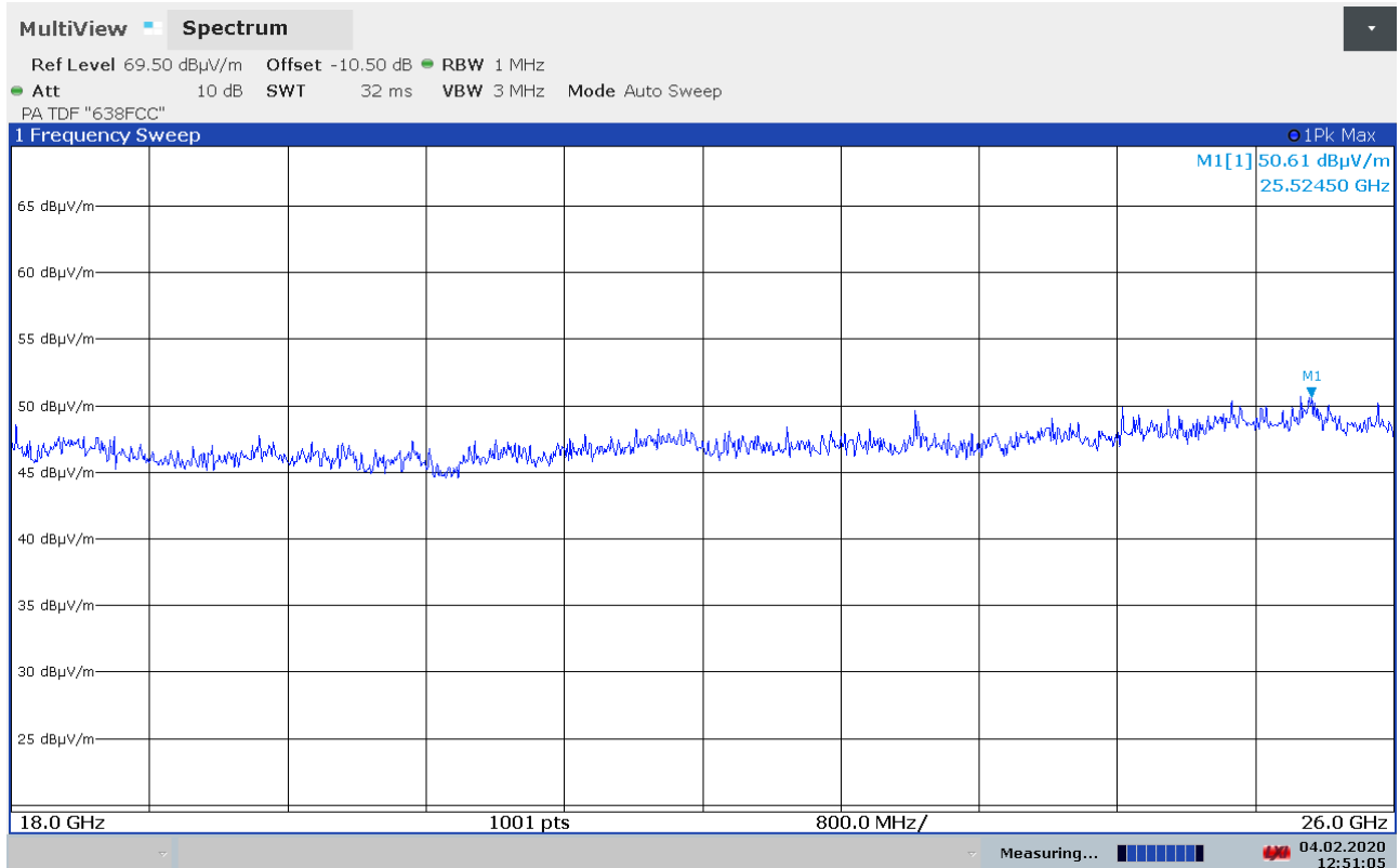
Radiated Emissions, 18 -26 GHz, 2462 MHz, VP, 802.11b, 11Mbps, @1m
