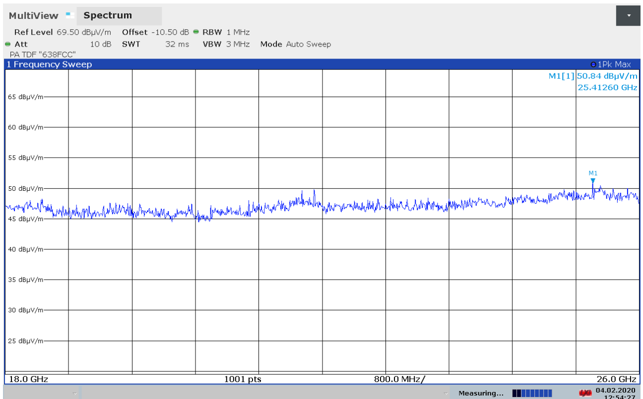
Radiated Emissions, 18 -26 GHz, 2437 MHz, HP, 802.11n, MCS7, @1m
