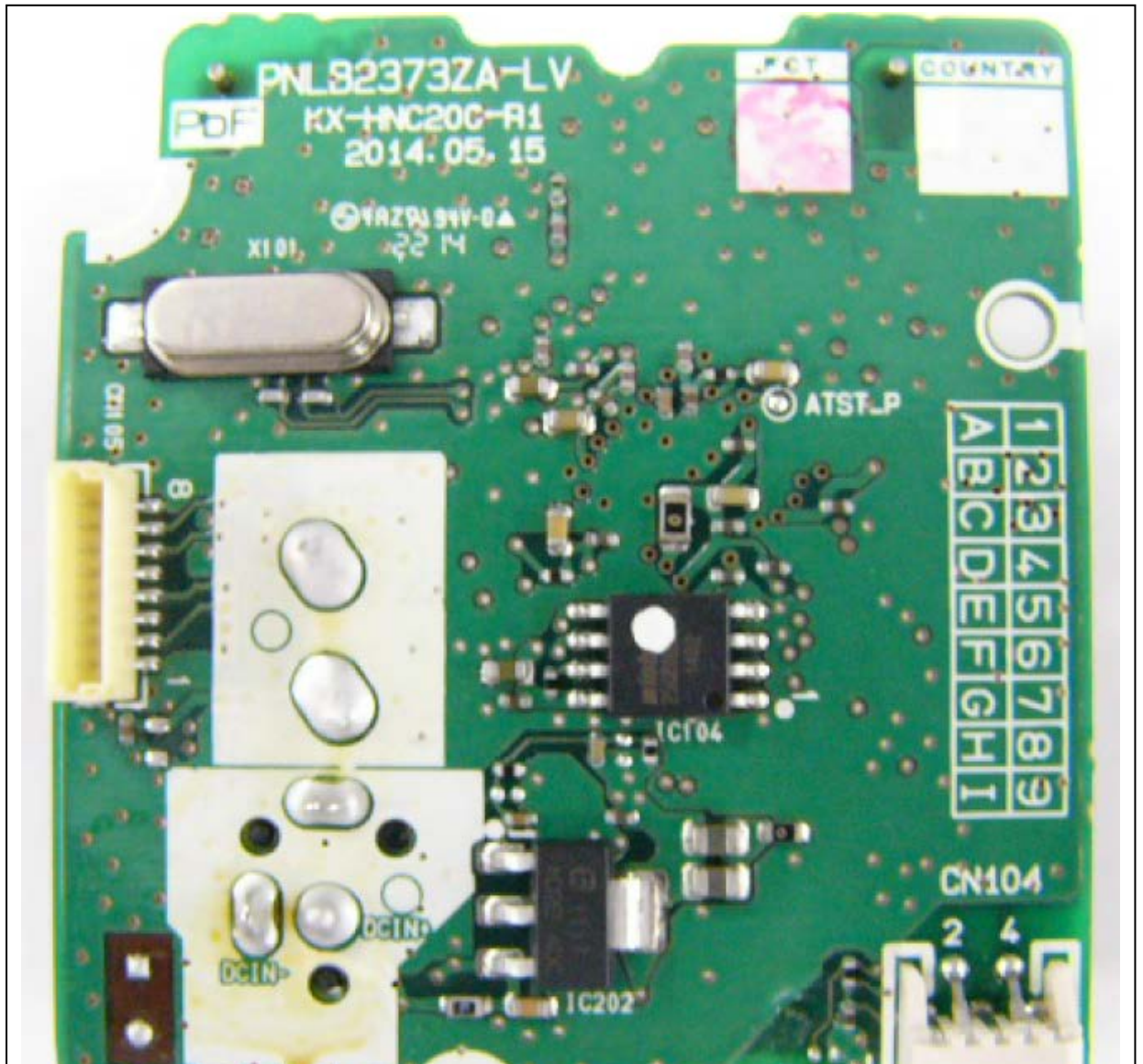
Main Board 2 (Downside)
