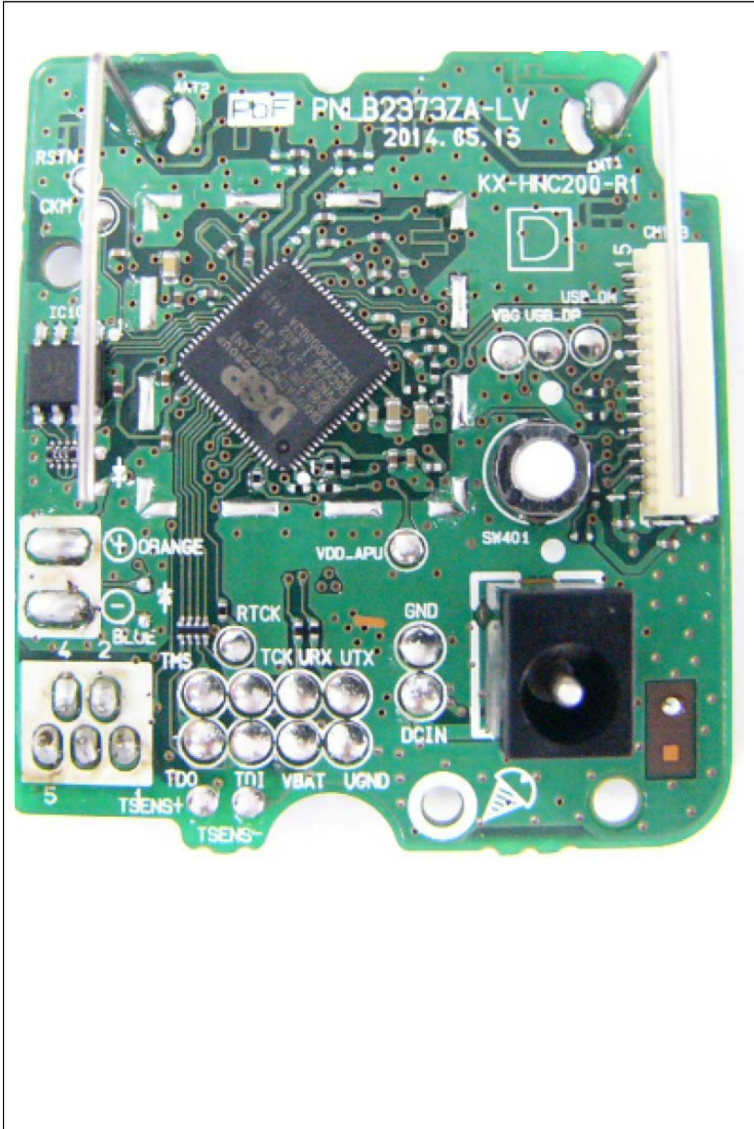
Main Board (Upside)
