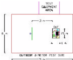
Figure 7. Dimensions of Outdoor Test Site
