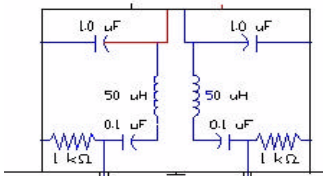
Figure 5. LISN Schematic Diagram
