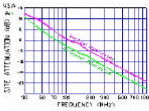
Figure 9. Normalized Site Attenuation Curves (H&V)
