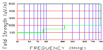
Figure 12. Restricted band harmonics and spurious limits.
