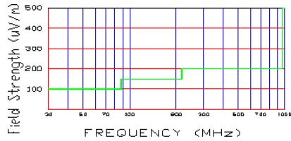
Figure 11. Restricted band harmonics and spurious limits.
