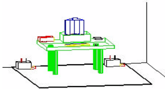
Figure 2. Line Conducted Emission Test Set-Up
