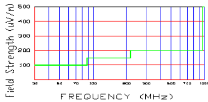
Figure 10. Restricted band harmonics and spurious limits.
