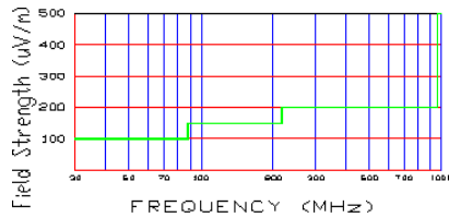
Figure 13. Restricted band harmonics and spurious limits.
