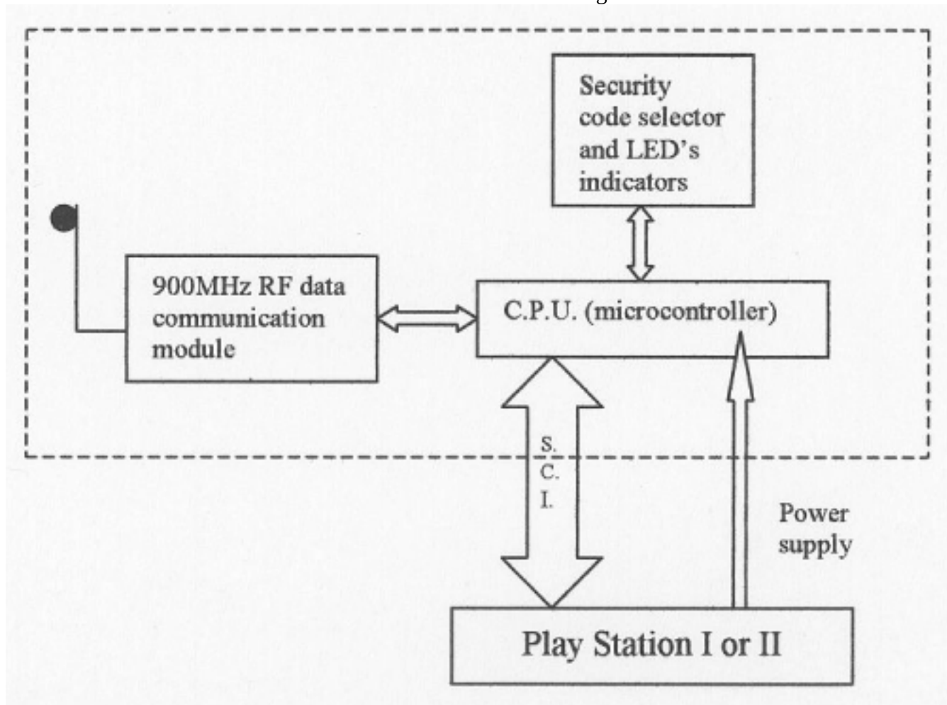
900MHz Base Unit Block Diagram
