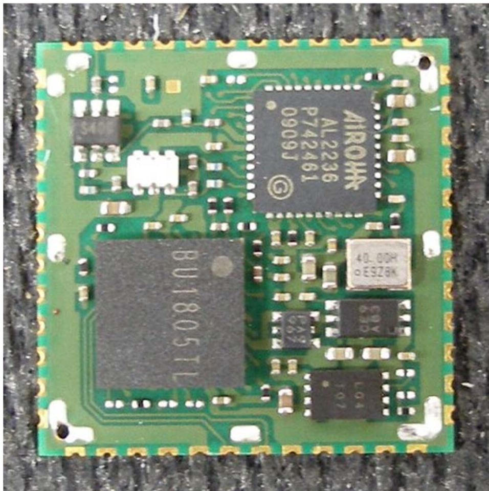
Side A without Shield
