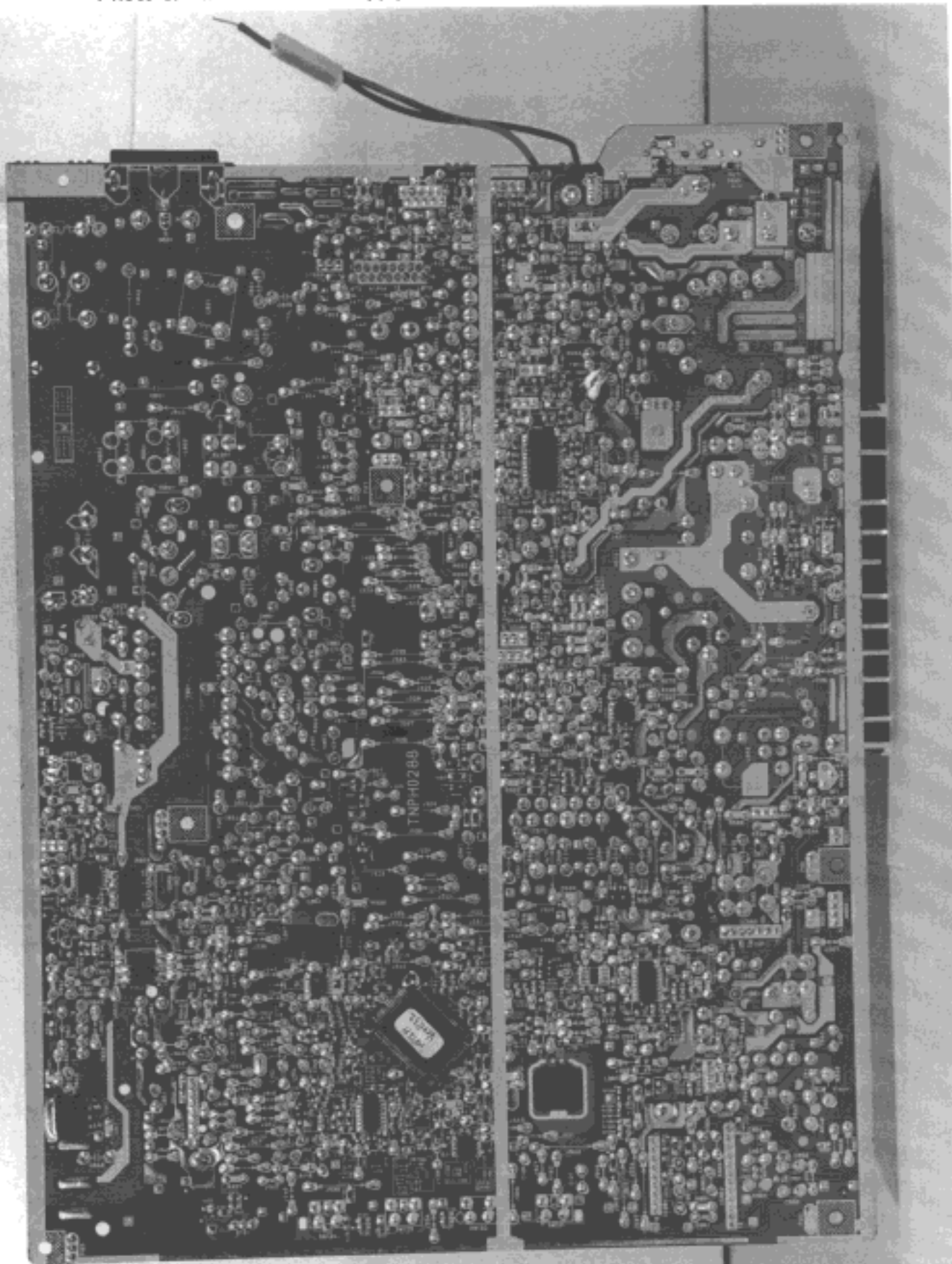
Photo 8. Main & Power Supply PCB of TX-D9S55NM (Reverse Side)
