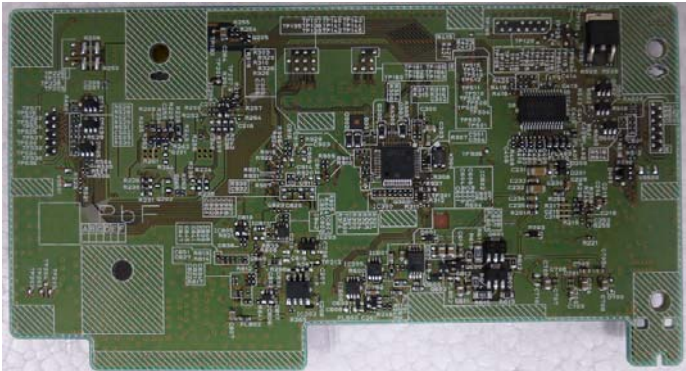
Fig.3 without Shield(Back)
