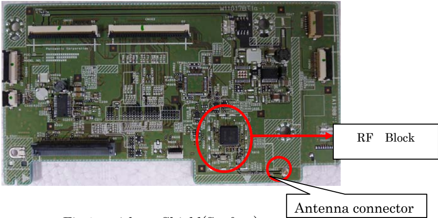
Fig.2 without Shield(Surface)
