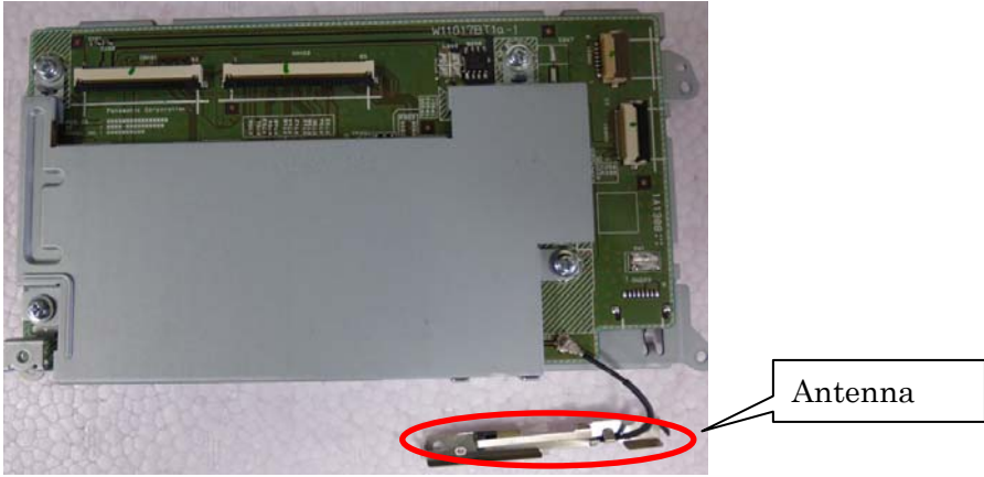
Fig.1 with Shield
