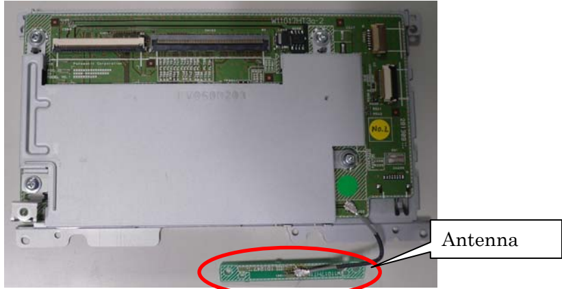
Fig.1 with Shield
