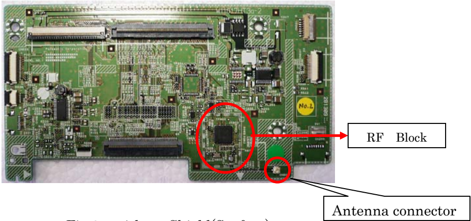
Fig.2 without Shield(Surface)
