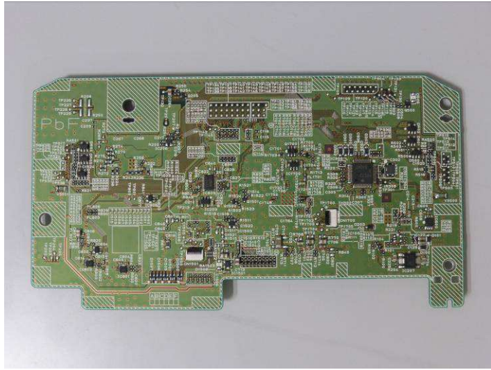
Fig.3 without Shield(Back)
