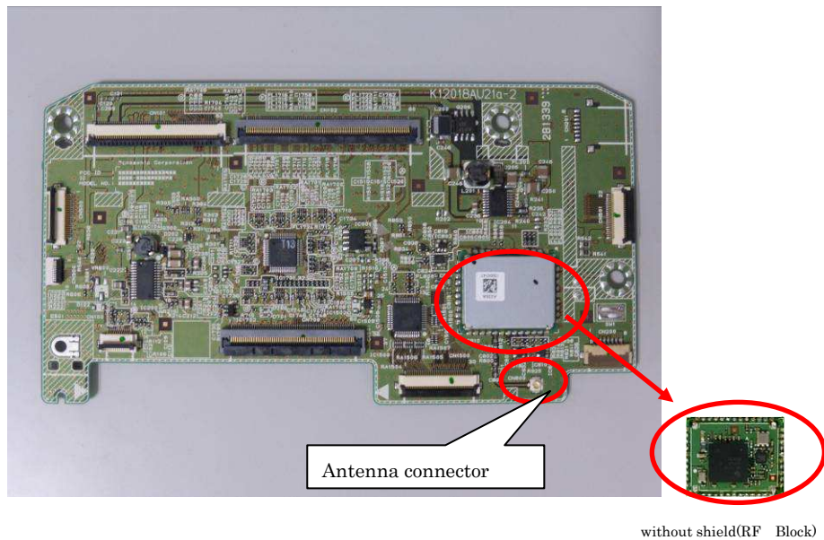
Fig.2 without Shield(Surface)
