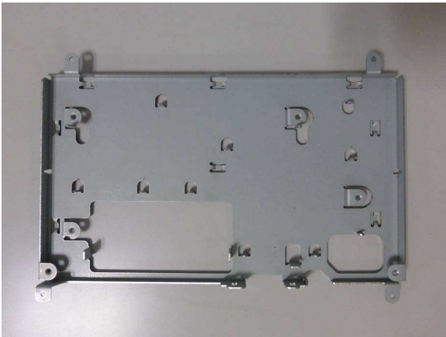
Fig.4 Bottom Plate
