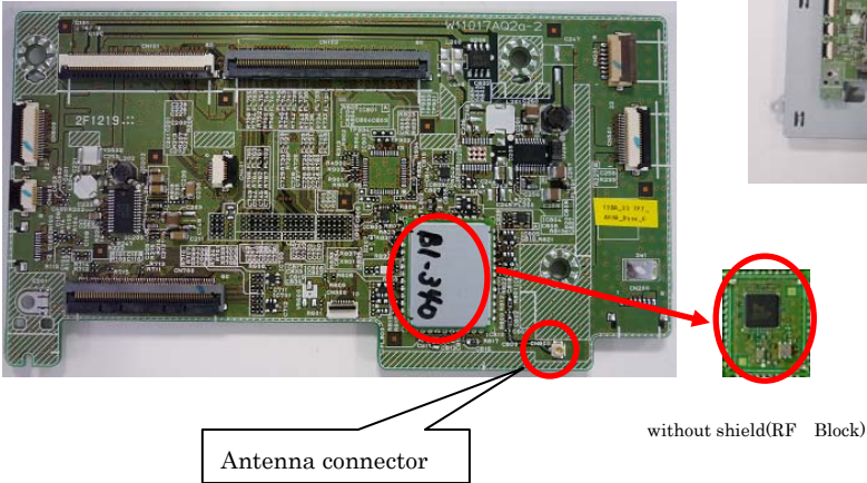
Fig.2 without Shield(Surface)
