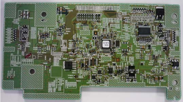
Fig.3 without Shield(Back)
