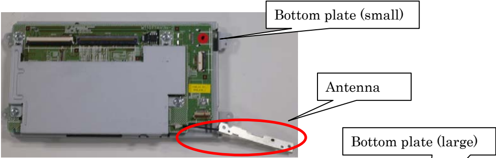
Fig.1 with Shield
