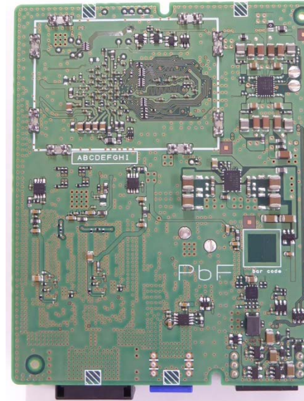
Back side (without shielding case)
