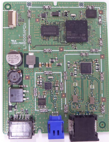
Surface side (without shielding case)
