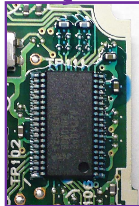
125kHz Receiver Block
