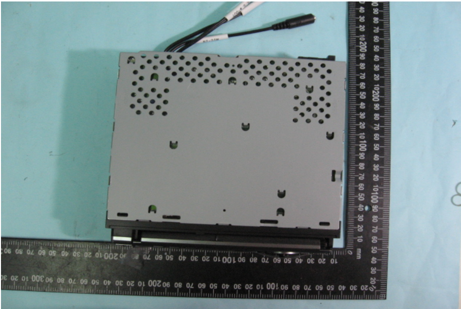
6. Top View of Car Radio
