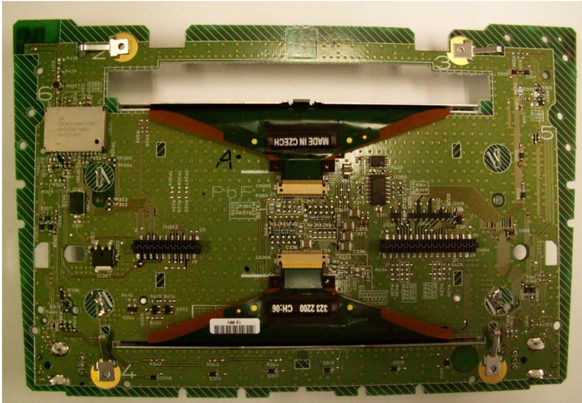
Rear of BT Module Board
