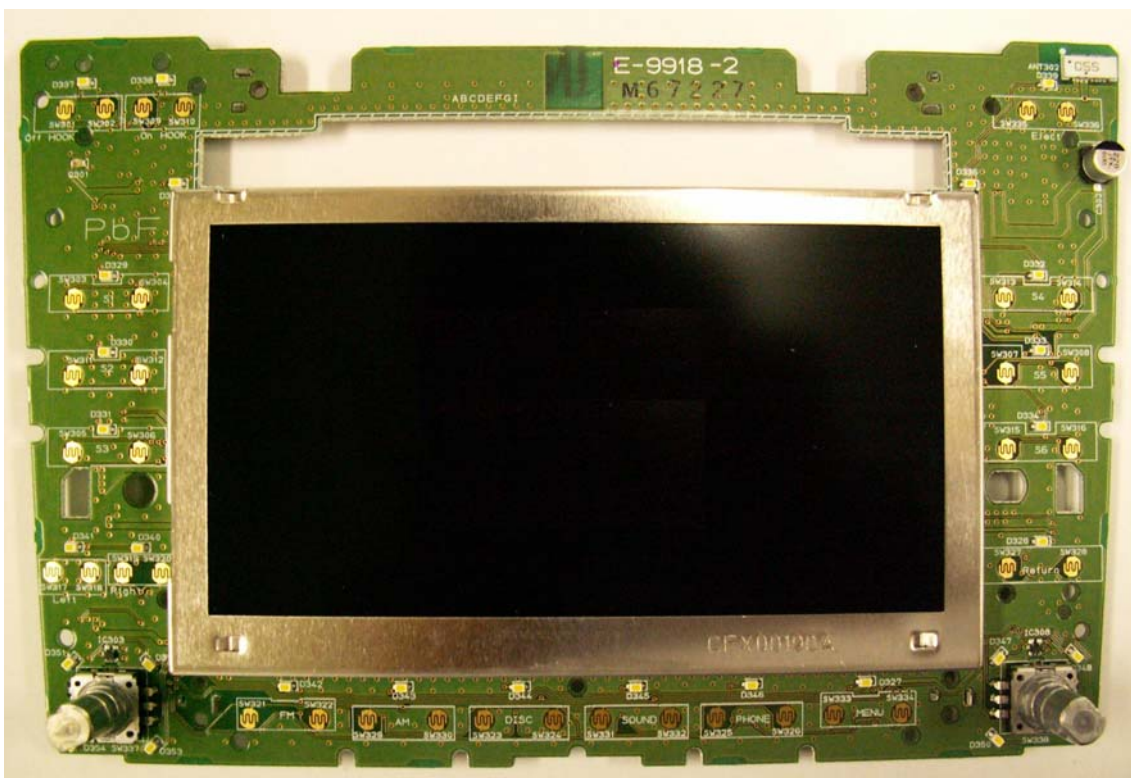
Front of BT Module Board with Display
