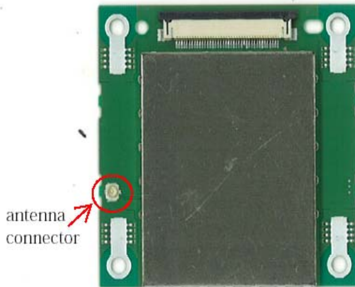
Front Side of Module with Shield
