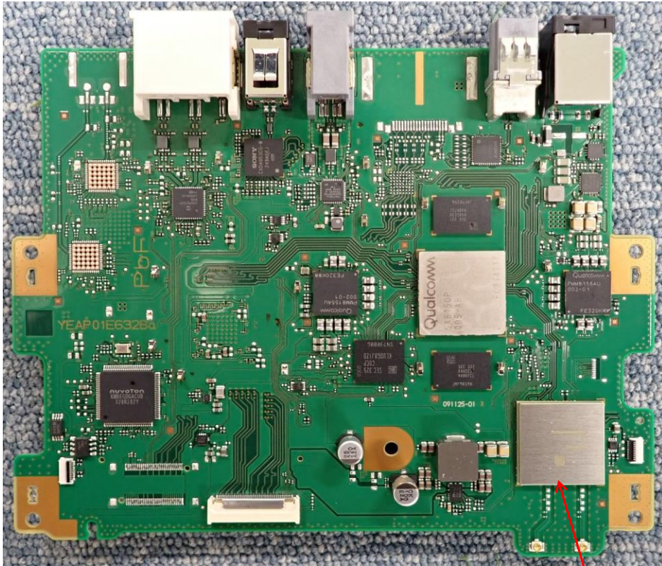
Wireless module
