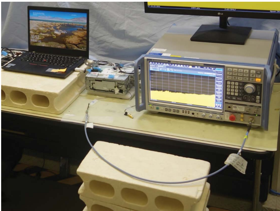
Photograph 6: Set-up for Antenna Port Connected Test, EUT ports
