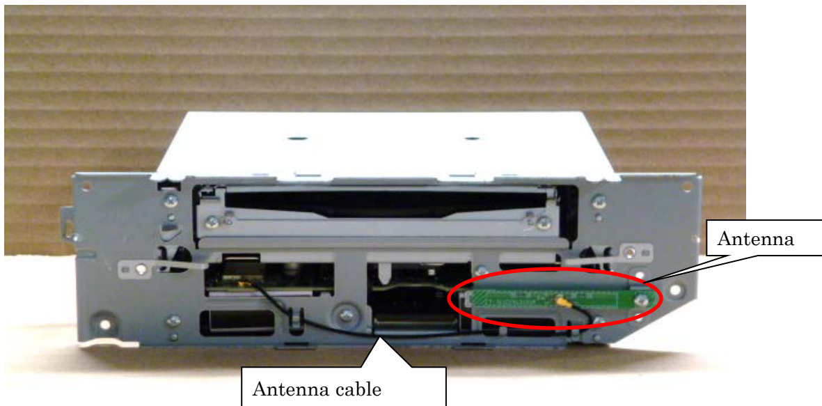
Fig.2 Without Display ASSY
