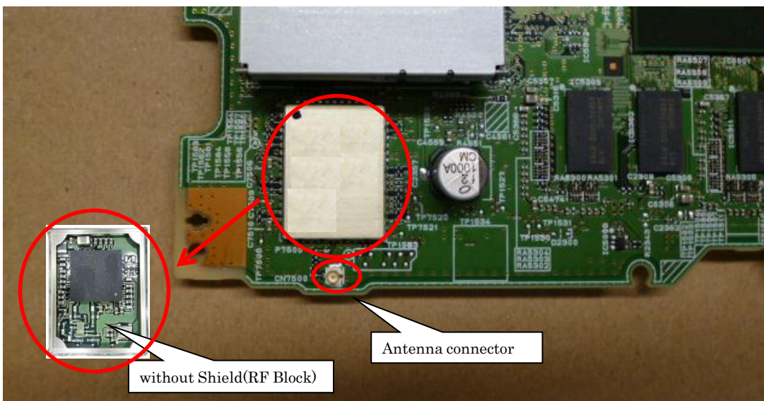
Fig.5 RF Block
