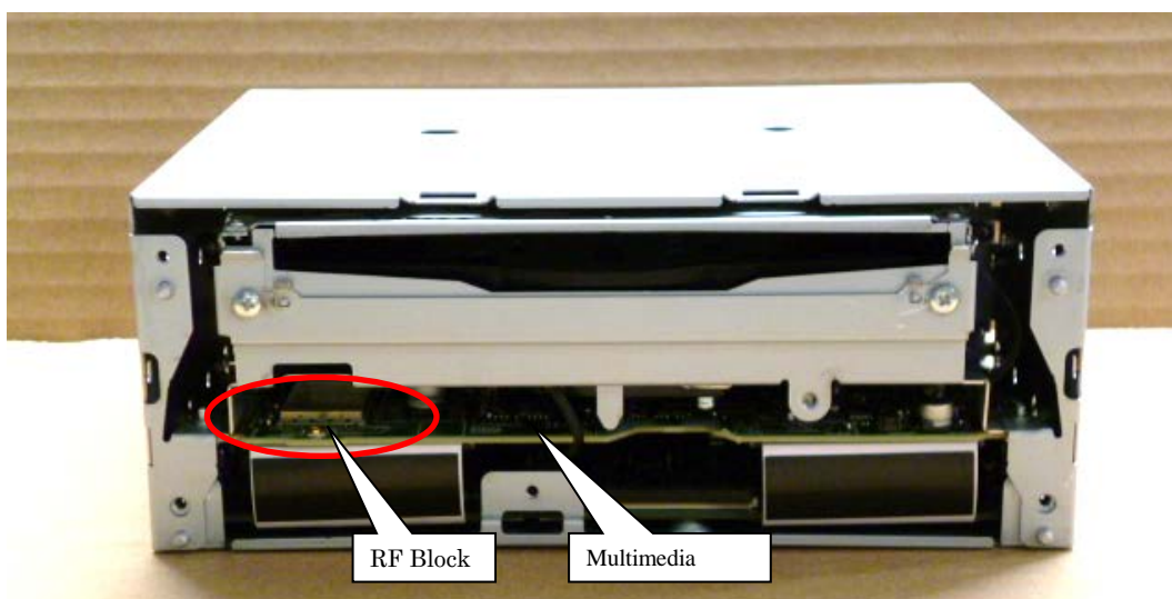
Fig.3 Without Front Plate
