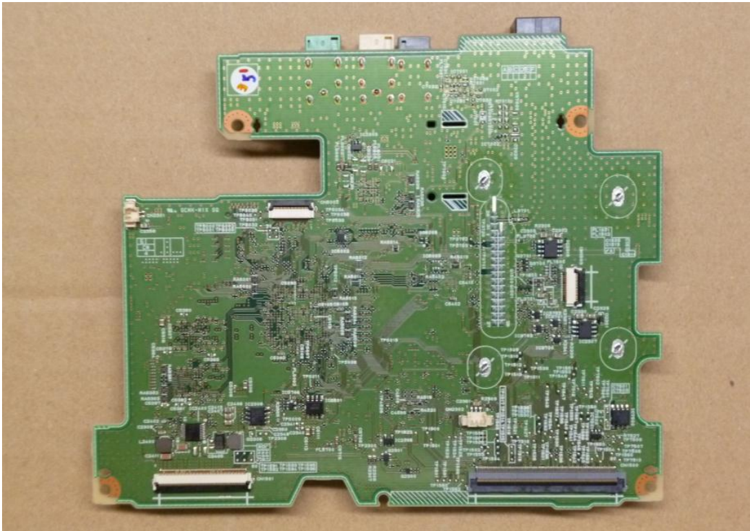
Fig.6 Multimedia PCB (Back side)
