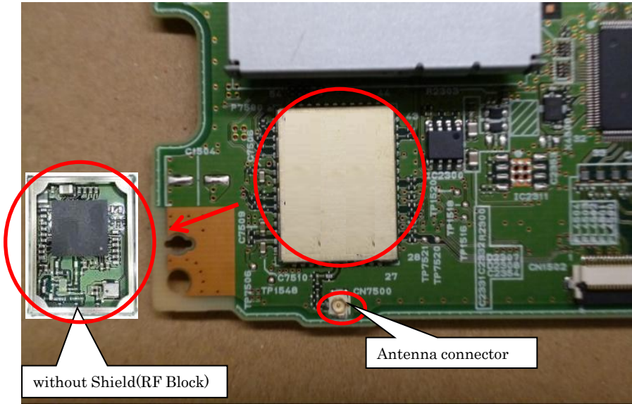
Fig.5 RF Block
