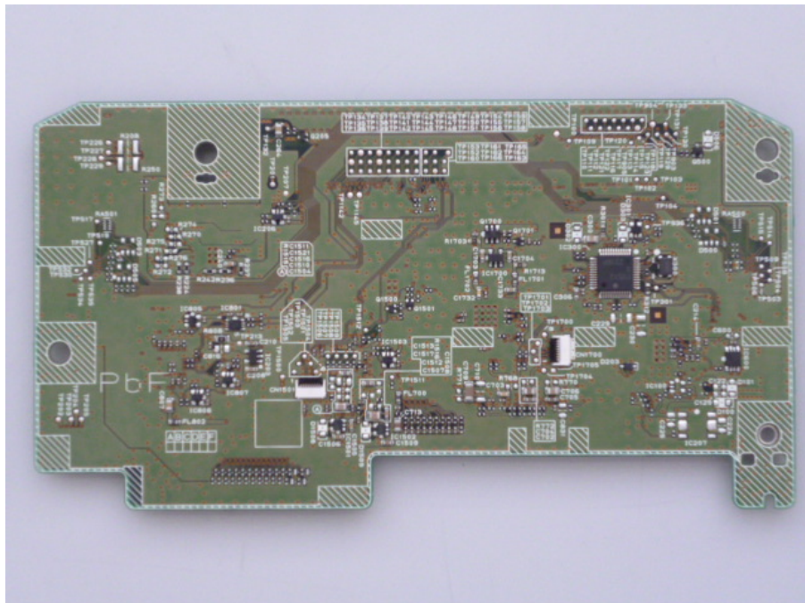
Fig.6 PCB (Back)
