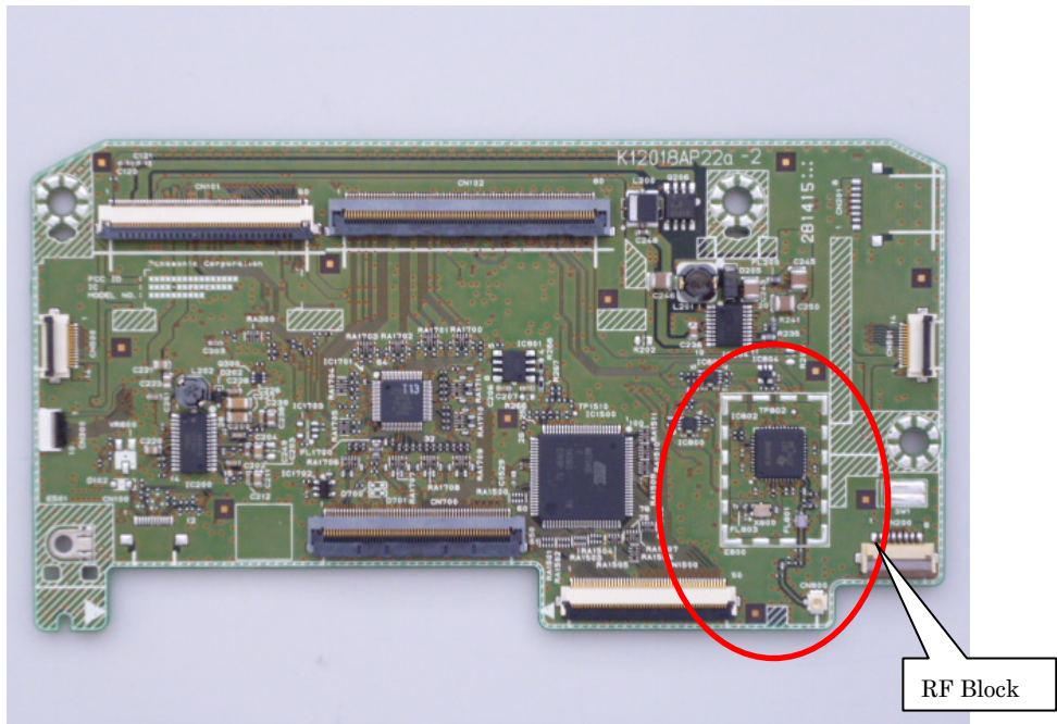
Fig.5 PCB (Surface)
