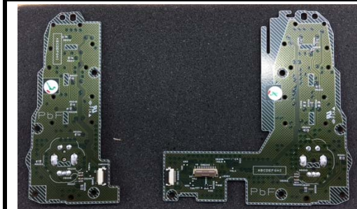
[PANEL PCB / Solder Side]
