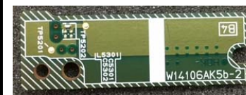
[TFT PCB / Surface Side] (Including BT)
