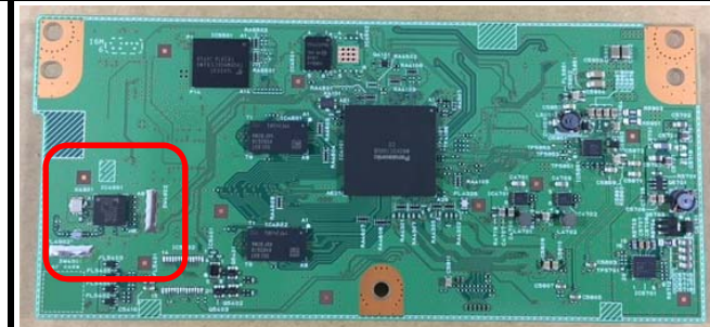
[TFT PCB / Surface Side] (Including BT)
