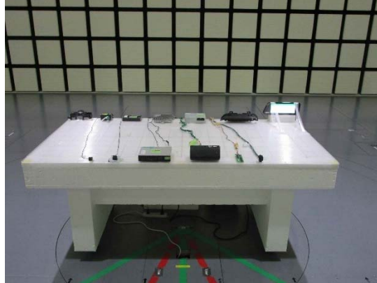
Rear(Below 1 GHz)
