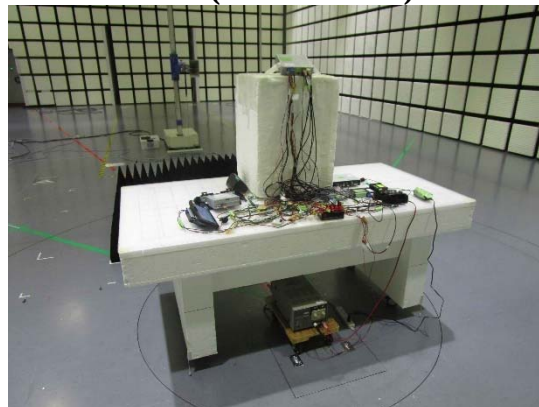
Rear(Above 1 GHz)
