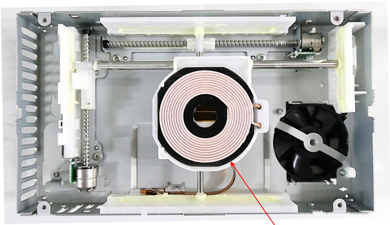
Primary Coil
