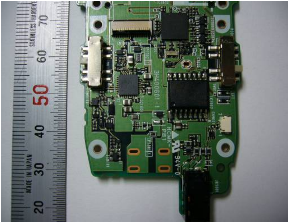
12) Main Board PCB View 7
