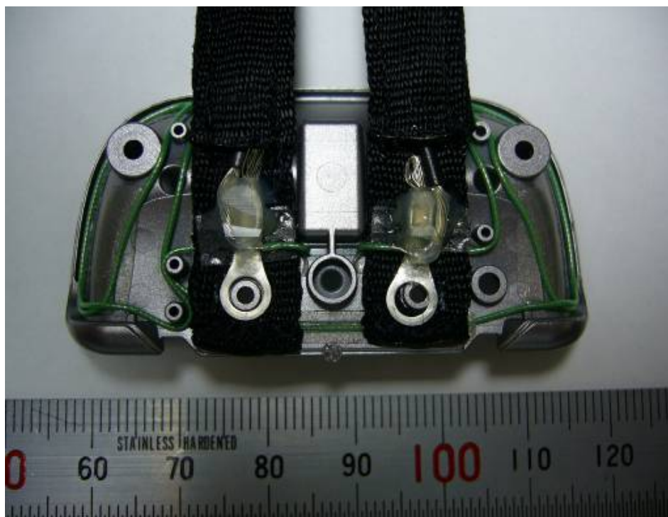
20) Loop Antenna Block View 4
