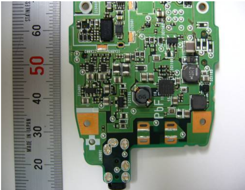
10) Main Board PCB View 5
