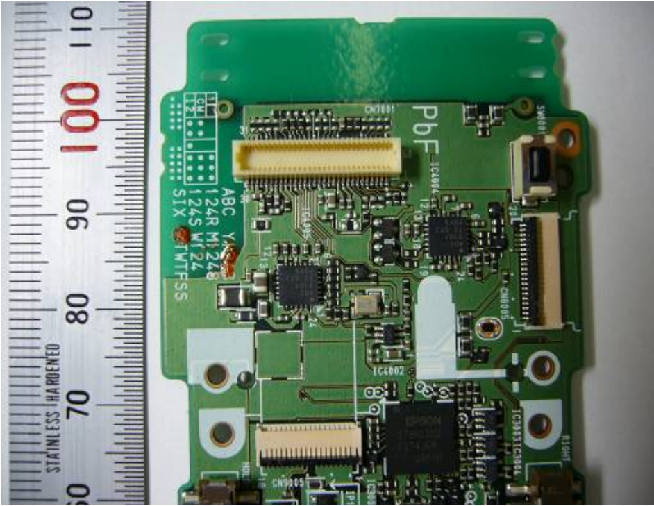
11) Main Board PCB View 6
