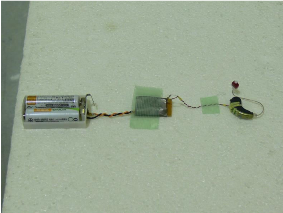
Photograph 2: Set-up for Radiated Emission of Transmitter, EUT and Test Jig, Configuration 2
