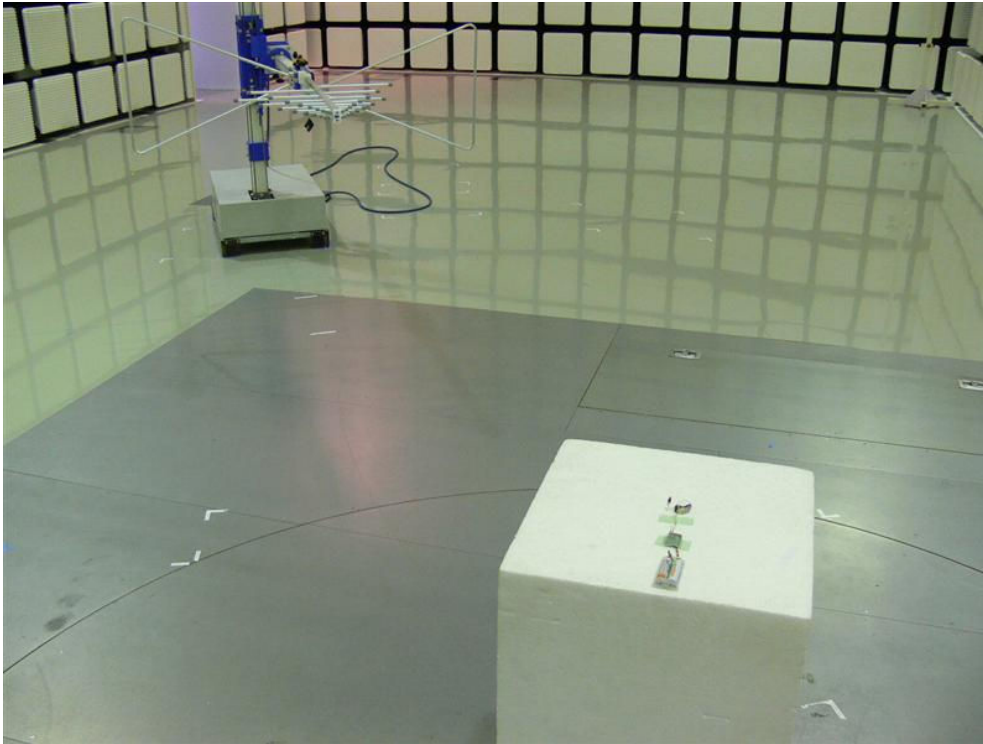
Photograph 4: Set-up for Radiated Emission of Transmitter, above 30MHz
