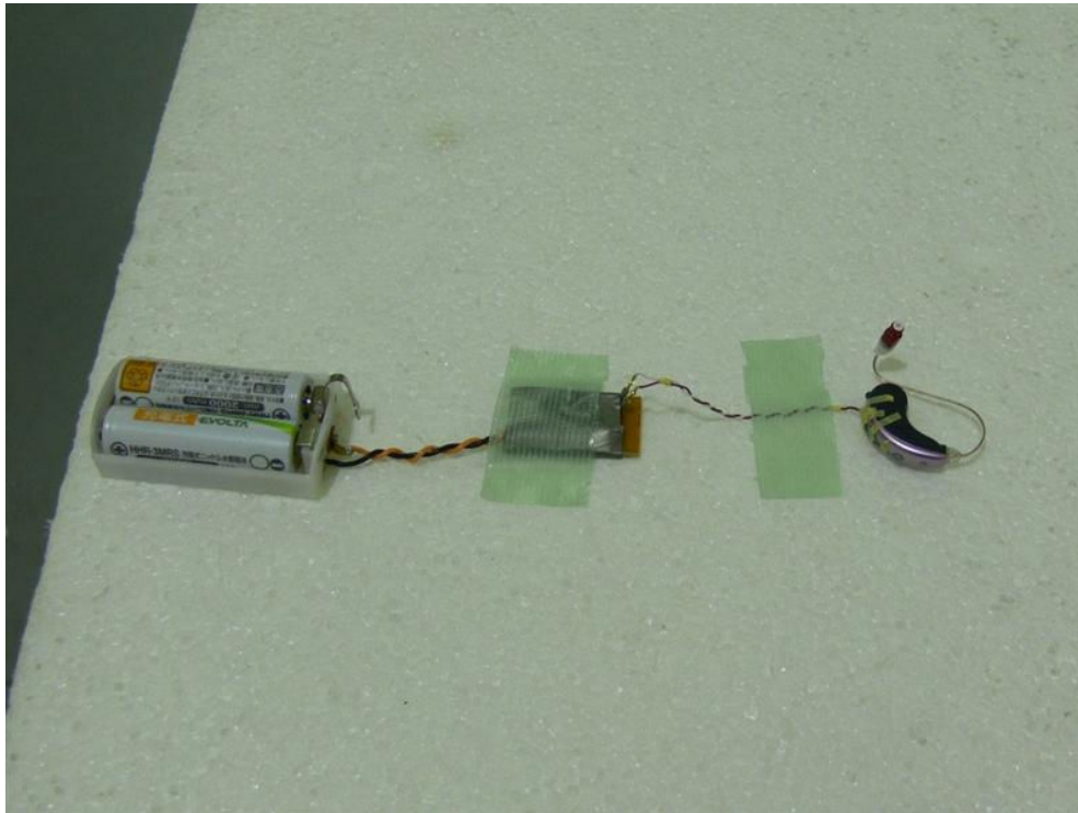
Photograph 1: Set-up for Radiated Emission of Transmitter, EUT and Test Jig, Configuration 1
