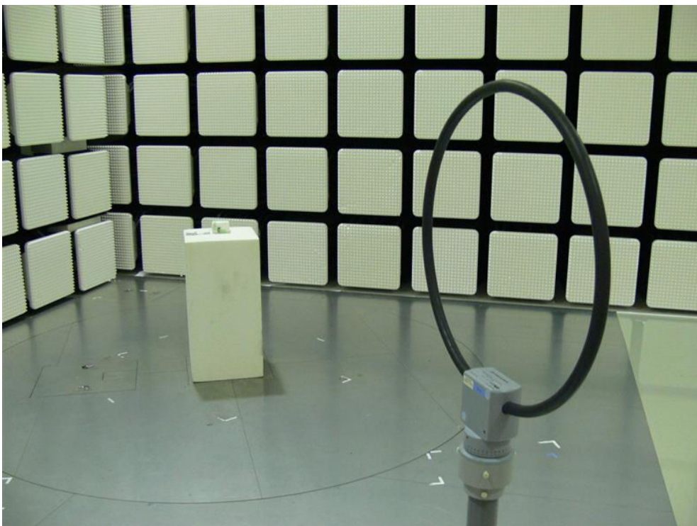
Photograph 3: Set-up for Radiated Emission of Transmitter, below 30MHz
