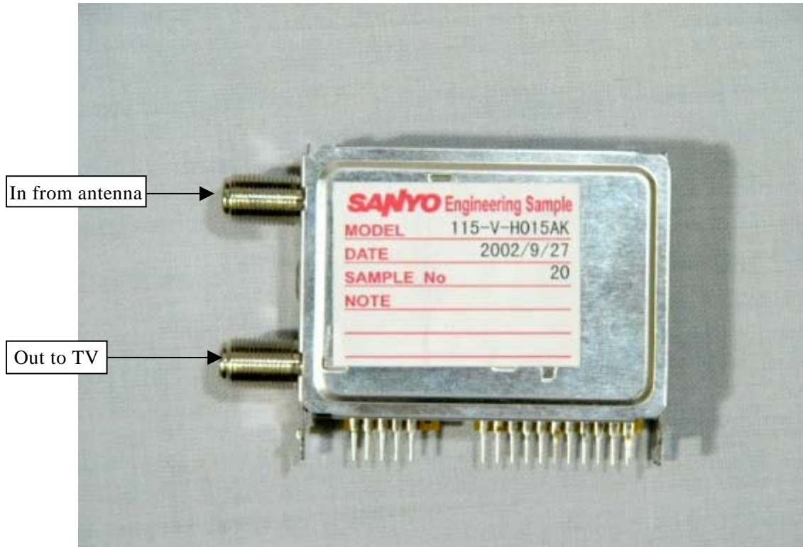
Tuner (115-V-H015AK: Top view)
